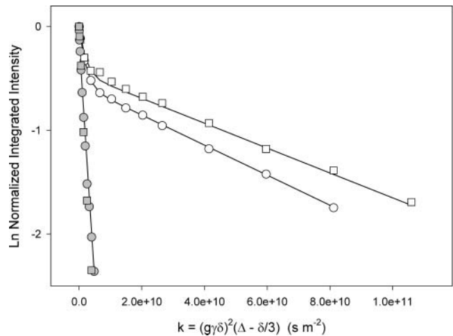
FIGURE 7 Stimulated echo intensity decays as a function of DMPE-PEG 2000 concentration in STE PFG ^1\text{H} NMR spectra (35°C) of magnetically aligned DMPC/DHPC ( q = 4.5 ) bicelles plus various levels of either DMPE-PEG 2000 or free (i.e., nonhydrophobically modified) PEG 2000. Gradient amplitude 244 \text{ G cm}^{-1} . (Open circles) 1 mol % DMPE-PEG 2000, \Delta = 615 \text{ ms} , D_{\text{PEG}} = 1.35 \times 10^{-11} \text{ m}^2\text{s}^{-1} . (Open squares) 2 mol % DMPE-PEG 2000, \Delta = 615 \text{ ms} , D_{\text{PEG}} = 1.15 \times 10^{-11} \text{ m}^2\text{s}^{-1} . (Shaded circles) 1 mol % free PEG 2000, \Delta = 60 \text{ ms} , D_{\text{PEG}} = 5.00 \times 10^{-10} \text{ m}^2\text{s}^{-1} . (Shaded squares) 2 mol % free PEG 2000, \Delta = 60 \text{ ms} , D_{\text{PEG}} = 5.23 \times 10^{-10} \text{ m}^2\text{s}^{-1} . DMPE-PEG 2000 diffusion coefficients were obtained using Eq. 4, the appropriate values of X_{\text{DHPC}} , X_{\text{PEG}} , and the relaxation times in Table 1. Free PEG 2000 diffusion coefficients were obtained using Eq. 1.
