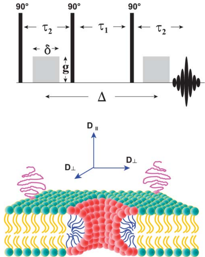
FIGURE 3 (Top) Stimulated echo (STE) pulsed field gradient (PFG) NMR sequence (Tanner, 1970). The phases of the three 90^\circ radio frequency pulses and of the receiver are cycled to eliminate unwanted echoes (Fauth et al., 1986). During the first delay time \tau_2 , a gradient pulse of amplitude g and duration \delta encodes the spins according to their position along the direction of the applied magnetic field gradient, in this case along the z direction. The spin magnetization is stored along the z direction during the second delay time \tau_1 to take advantage of the case T_1 > T_2 , thereby permitting longer diffusion times \Delta . During the third delay time \tau_2 , the second gradient pulse decodes according to position along the direction of the applied gradient. The intensity of the stimulated echo that forms at a time \tau_2 after the third radio frequency pulse decreases with increasing diffusion during the time as per Eq. 1. A train of three identical gradient pulses with a repetition period of \tau_1 + \tau_2 was imposed before the STE PFG NMR sequence to equalize eddy current effects during the two transverse evolution periods (Gibbs and Johnson, 1991). (Bottom) Schematic cross section of a DMPC/DHPC bicelle in the perforated lamellae model morphology. DMPC (green-yellow) forms the lamellar bilayer region, whereas DHPC (red-blue) is sequestered into highly curved toroidal "holes" forming perforations in the lamellae. For amphiphiles resident within or upon the lamellar bilayer, such as the PEG-lipid (magenta) shown with its PEG headgroup extending into the aqueous bathing medium, the molecule-fixed diffusion tensor is completely described in terms of D_{\parallel} and D_{\perp} , referring to diffusion in a direction parallel or perpendicular, respectively, to the normal to the plane of the bilayer. D_{\perp} corresponds, therefore, to lateral diffusion within the plane of the bilayer.
