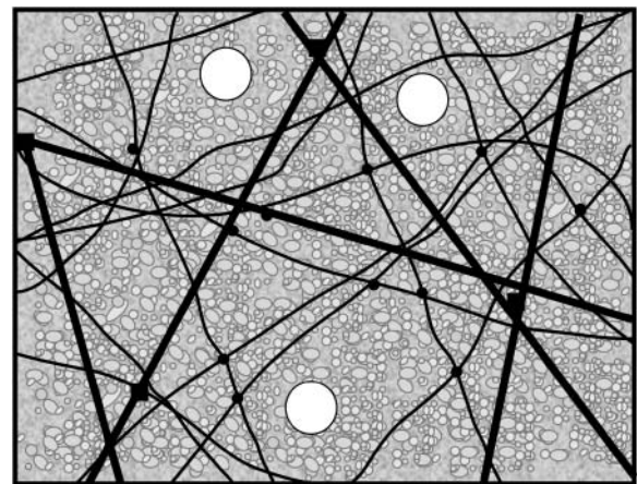
FIGURE 7 Sketch of the mechanically important structures in egg extract. F-actin, microtubules, and cytokeatin form a composite network stiffened by numerous cross-linking proteins ( solid circles and squares ). Protein-resistant micron-sized colloidal particles ( white circles ) do not interact with the elastic mesh; rather, they move within mechanically distinct microenvironments. The cytoskeleton is bathed in a concentrated protein solution, the cytosol, represented by the small macromolecules ( grayscale, in background ). This concentrated suspension increases the microscopic viscosity to \sim 20 times that of water.
