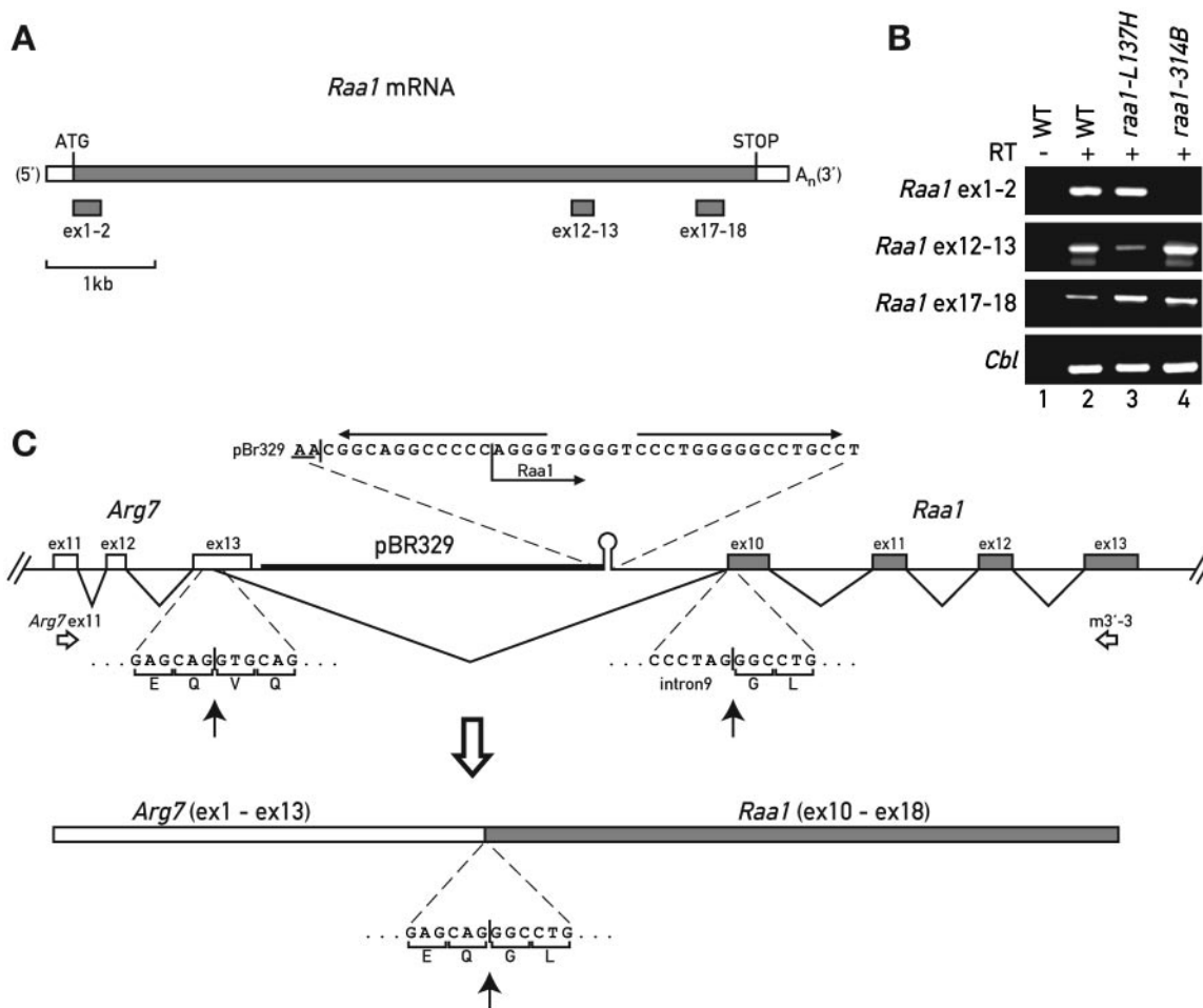
Figure 2. Expression of Raa1 in the mutants. (A) Schematic representation of the Raa1 mRNA with the fragments amplified in the RT-PCR analysis. (B) RT-PCR analysis with RNA from the wild-type (WT), raa1-314B and raa1-L137H , for three parts of Raa1 (panel A) and the Cbl transcript as a control. The + or – signs indicate whether reverse transcriptase was included (lanes 2–4) or omitted as a control (lane 1). (C) The 3' part of Raa1 is expressed as a fusion to Arg7 in raa1-314B . The structure of the genomic DNA in raa1-314B is shown with the last exons of Arg7 (open bars), a fragment of the cloning vector pBR329 from pARG7.8 (thick black line), the 3' part of Raa1 intron 9 (thin black line) and the exons of Raa1 (shaded bars). The sequence of a short hairpin-loop created at the insertion site by duplication of a 15 bp sequence of Raa1 is indicated above the scheme. A cryptic donor site in exon 13 of Arg7 (black arrow) and the acceptor site of exon 10 of Raa1 (black arrow) are used for splicing across the pBR329 sequence to generate an in-frame fusion transcript as indicated at the bottom.
