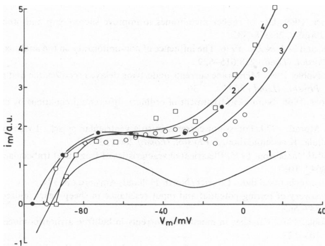
FIGURE 10 Comparison of input curve 1 and output curve 2 ( \bullet ) of Fig. 6B with experimentally determined curves of background current (3: eyefit of \circ ; 4: eyefit of \square ) from Giles and Noble (1976), the latter shifted by 13.9 \text{ mV} to the left along the voltage axis and scaled to give approximate amplitude fit with curve 2 (see text). All currents in arbitrary units.
