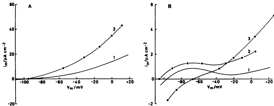
FIGURE 6 Modification of current/voltage curves. (A) evaluation of Fig. 4; curve 1, input curve (sum of Eqs. 9a and b with P_K = 10^{-6} cm s ^{-1} and P_{Na} = 10^{-8} cm s ^{-1} ); curve 2, output curve constructed as described in text. (B) evaluation of Fig. 5; curve 1, input curve (sum of Eqs. 9a and b with P_K according to Eq. 10 and P_{Na} = 10^{-8} cm s ^{-1} ); curves 2 and 3, output curves obtained from Fig. 5A and 5B , respectively.
