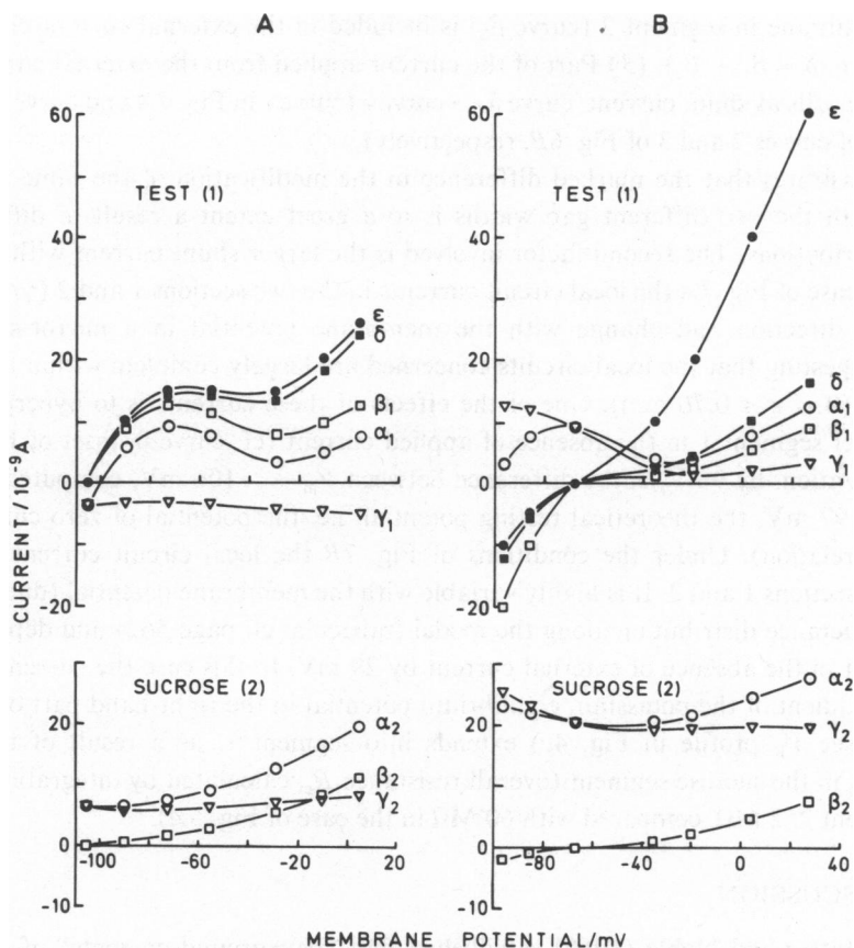
FIGURE 7 Current components of test compartment (top, 1) and of adjoining region of sucrose compartment (bottom, 2). A , gap width 0.8 mm; B , gap width 0.4 mm. Membrane current ( \circ ) in each of the two compartments ( \alpha_1 and \alpha_2 , respectively) is composed of current from external current source ( \square ; \beta_1 and \beta_2 , respectively) and local circuit current ( \nabla ; \gamma_1 and \gamma_2 , respectively): \alpha_1 = \beta_1 + \gamma_1 ; \alpha_2 = \beta_2 + \gamma_2 . Currents obtained by integration as described in the text and plotted against membrane potential in test compartment. Curve \delta ( \blacksquare ) in each top panel: sum of currents from external source from test and sucrose region ( \delta = \beta_1 + \beta_2 ); curve \epsilon ( \bullet ): measured current, i.e. curve \delta plus shunt current.
