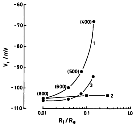
FIGURE 9 Dependence of computed resting potential ( V_r ) on shunt factor ( R_i/R_c ). Variations of R_i/R_c either by variation of gap width ( \bullet ; curves 1 and 3, widths in \mu\text{m} given in brackets), or by variation of R_i only ( \blacksquare ; curve 2, gap width 800 \mu\text{m} ). 1 and 2: potassium permeability ( P_K ) as described by Eq. 10; 3: P_K increased twofold.
