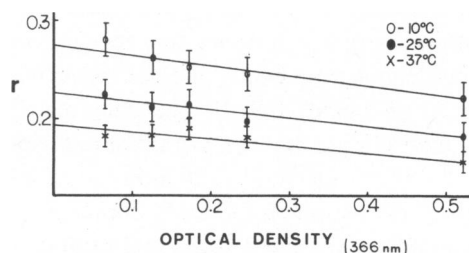
FIGURE 2 Anisotropy ( r ) of DPH fluorescence vs. optical density for several dilutions of delipidated (2.0 mol % Ca 2+ -activated ATPase) sarcoplasmic reticulum vesicles, at three temperatures.
