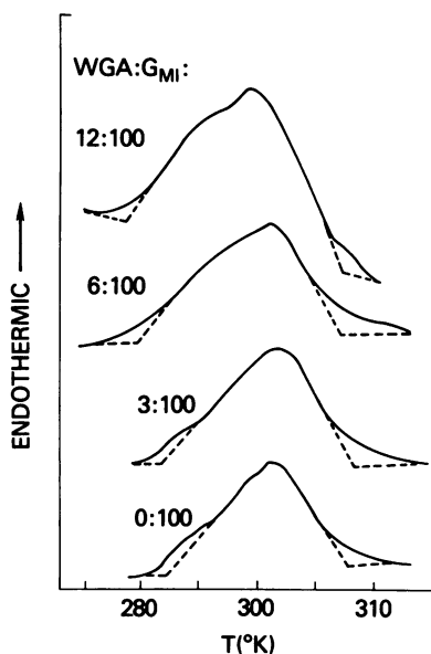
FIGURE 9 Heat uptake curves for G_{\text{MI}} -SOPC mixtures ( X_{\text{GM}_1} = 0.5 ) upon addition of WGA at molar ratios, WGA: G_{\text{MI}} , shown on the curves.
