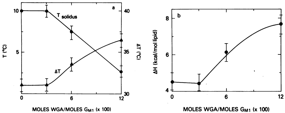
FIGURE 10 (a) Lowering of solidus ( \bullet ) and increase in phase transition width ( \blacktriangle ) in ^{\circ}\text{C} for ganglioside G_{M1} -SOPC mixtures ( X_{G_{M1}} = 0.5 ) upon addition of WGA. The system was suspended in phosphate buffer, pH 7.2, at a final concentration of 50 mM buffer. (b) Increase in transition heats of ganglioside G_{M1} -SOPC mixtures, upon addition of WGA.
