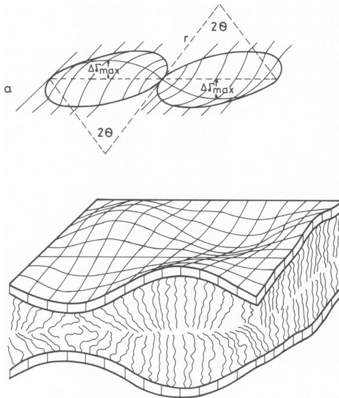
FIGURE 2 Breathing model of a lipid bilayer. (a) A swelling and an indentation, shaped like spherical caps.
