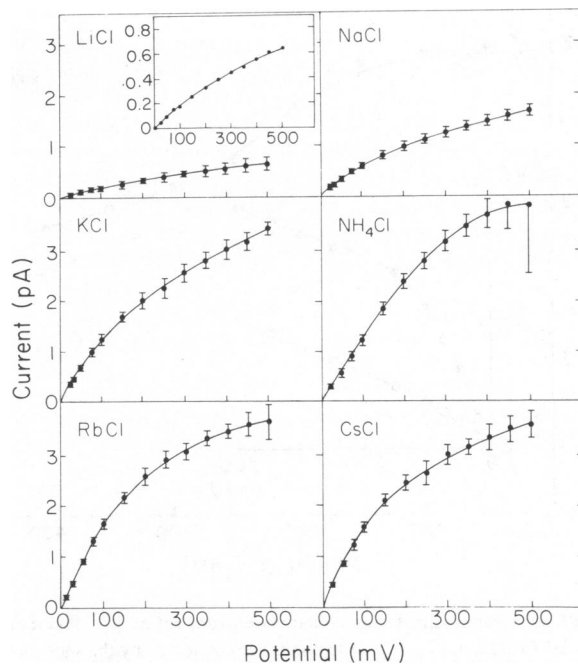
FIGURE 8 Gramicidin A single-channel current-voltage characteristics. Each point indicates the mean ( \pm SD) of the current. (The exceptionally large scatter of the data with 0.1 M NH 4 Cl, at 500 mV reflects the difficulty of the measurement. Only 43 transitions were collected.) To facilitate the visual comparison of different records, they are all drawn to the same scale (except for the inset illustrating the LiCl data at a 3.25 \times magnification). The solid curves are drawn by hand. 0.1 M salt; GMO, 25°C.
