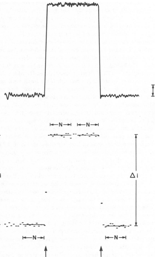
FIGURE 3 The data-collecting scheme. A single channel is drawn schematically in the top part. The bar at right illustrates the discrimination level; its magnitude is determined by looking at the channels on the oscilloscope screen. The digitized record corresponding to this channel is illustrated in the bottom part. The digitized data are transiently stored in a circular buffer in the computer memory. Two successive points (denoted by arrows) differ by more than the discrimination level at the channel opening and at the channel closing. Each of these events trigger the data-collection routine. Beginning with the last data point before the discrimination level was exceeded, the computer searches a fixed number N ( 5 \leq N \leq 10 ) points back in the buffer. If these all differ by less than the discrimination level, the pretransition current level is termed well-defined and its value is obtained as the average value of the N points (illustrated by the thin horizontal line). The posttransition level is then determined. The point at which the discrimination level was exceeded and the next are disregarded. The next N points are then used to determine whether the level is well defined. If both levels are well defined the current transition is called well defined. The value of the posttransition current level is again evaluated, as the average value of the N points, and the height of the current transition is determined as the absolute value of the difference between the posttransition level and the pretransition level.
