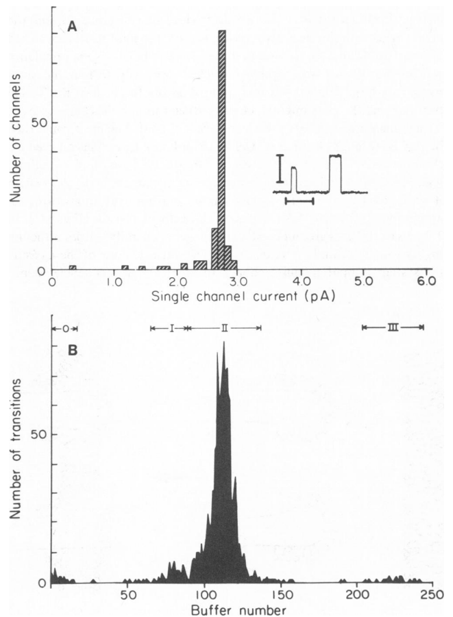
FIGURE 4 Amplitude histograms for gramicidin A single channels in 0.1 M, RbCl, with 300 mV applied potential, R_f = 10^9 \Omega , filter = 50–100 Hz, 25°C. A , histogram compiled from 119 single channels. The mode of the distribution is 2.74 pA. For the whole histogram \bar{i} = 2.66 \pm 0.34 pA [mean \pm SD ( n = 119 )], for the major peak in the histogram \bar{i} = 2.75 \pm 0.05 pA ( n = 107 ). The inset illustrates directly the existence of several difference channel sizes. The calibration bars denote 2pA, vertically, and 1 s, horizontally. B , histograms of single-channel current transitions compiled from 10 individual experimental records analyzed on-line on the computer. An increment of 1 in the buffer corresponds to a current increment of 0.024414 pA, the abscissae in the top and bottom part of the figure are thus aligned. The mode of the distribution is 2.76 pA. The four regions, labeled 0, I, II, III, illustrate the most conspicuous aspects of the histograms. 0 denotes current transitions where the data acquisition routine was triggered by a brief spike, such that the current returned to the base-line before the second level was to be determined. I denotes a population of channels with an amplitude less than the most commonly seen amplitude (see the inset in the top part of the diagram). II denotes the major population of channels. III denotes a small number of events where two channels opened simultaneously within the time-resolution determined by the filter setting. For the whole histogram \bar{i} = 2.74 \pm 0.58 pA ( n = 1257 ). For the major population, II, \bar{i} = 2.75 \pm 0.18 pA ( n = 1130 ), for population III, \bar{i} = 5.50 \pm 0.23 pA ( n = 21 ), and for population I, \bar{i} = 1.99 \pm 0.13 pA ( n = 61 ). The standard deviations are larger than for the manually compiled histogram. This is instrumental, as the mean square deviation from zero in population 0, is 0.15 pA ( n = 21 ).
