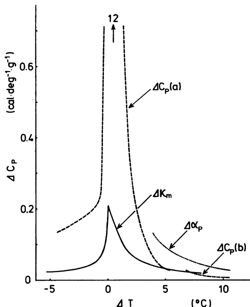
FIGURE 5 Anomalies of the specific heat in the vicinity of the transition temperature. ---, \Delta C_p (a) from reference 1 and ····, \Delta C_p (b) from reference 27 were measured by a differential scanning calorimeter. The estimation of the specific-heat anomaly from \Delta\kappa_m , —, and \Delta\alpha_p , · · · ·, (30) was performed using Pippard's relation (Eqs. 7 and 8). Appropriate base lines were assumed for \Delta C_p (b) and \Delta\alpha_p extrapolating from more than 20°C above the transition temperature.
