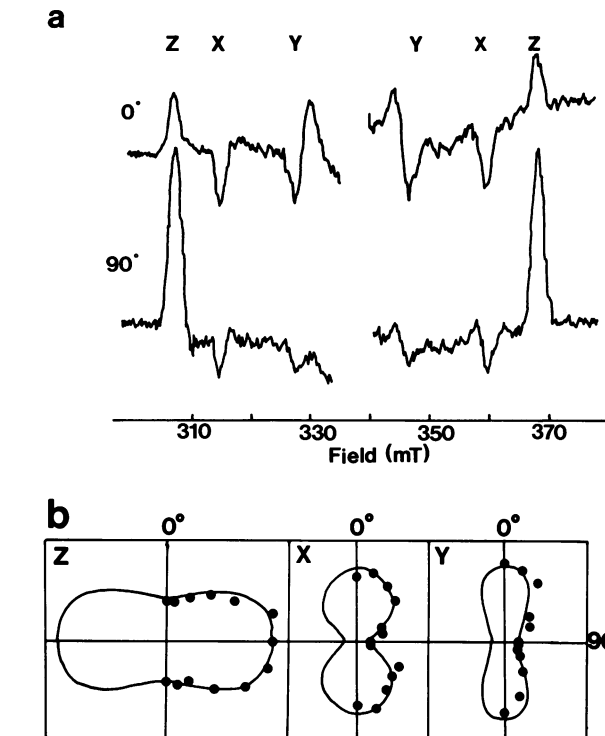
FIGURE 2 The orientation dependence of the P680 triplet in isolated PS II reaction centers. The sample, which was partially dried on mylar sheets, was submerged in sodium dithionite (20% in 200 mM glycine pH 9.0) under an O_2 free argon atmosphere for 5 min in darkness at 22^\circ C . Instrument settings were as follows: temperature, 4.2 K; microwave power 35 dB down from 200 mW, modulation amplitude 20 G. Spectra were recorded under illumination using white light from an 800 watt projector. (a) EPR spectra recorded when the mylar sheets were parallel ( 0^\circ ) and perpendicular ( 90^\circ ) to the magnetic field. (b) Polar plots of the ZXY features of the triplet signal.
