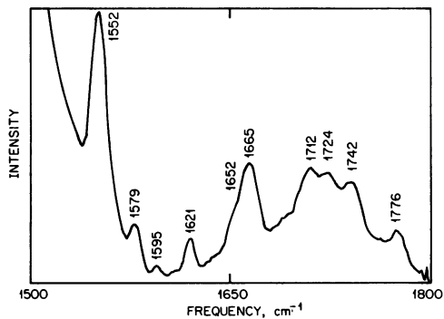
FIGURE 5 Raman spectrum in the 1,500–1,800 \text{cm}^{-1} region of gramicidin A in dioxane.
