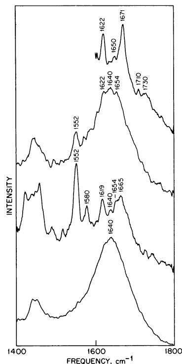
FIGURE 6 Raman spectra in 1,400–1,800 \text{cm}^{-1} region of gramicidin A in vesicles. (a) Vesicles in water, (b) gramicidin A in vesicle suspension after 10 min incubation at 45°C, (c) gramicidin A in vesicle suspension after 8–15 h incubation at 60°C and (d) dried sample of c.
