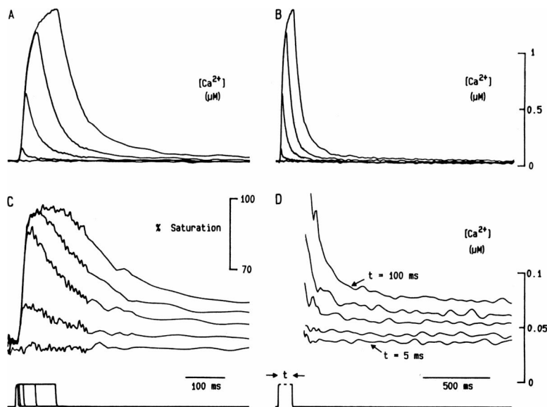
FIGURE 7 Calcium transients in a skeletal muscle fiber recorded simultaneously with antipyrylazo III and fura-2 for pulses of constant amplitude but varying duration. ( A and B ) [Ca^{2+}] records calculated from AP III absorbance signals at 700 nm. The same records are presented in A and B on different time scales. ( C ) Fura-2 percent saturation calculated from fura-2 fluorescence ratio signals recorded simultaneously with the AP III signals in A and B . Same time scale as in A . ( D ) [Ca^{2+}] records calculated from the fura-2 signals in C , presented on the same time scale as used for B . Because of the expanded [Ca^{2+}] axis used in D , the [Ca^{2+}] records were out of range during the pulses. When in range, the amplitudes of the “maintained” levels of [Ca^{2+}] after the pulses increased as the pulse duration ( t , bottom) was increased from 5 to 100 ms. The values of the fura-2 constants obtained for this fiber as in Fig. 6 and used in C and D were -R_{max} = -0.32 , k_{on} = 3.65 \times 10^8 M^{-1}s^{-1} , k_{off} = 24 s^{-1} ( -R_{min} = -2.00 , as in Fig. 6, legend). Fiber 370, 4.0 \mu m per sarcomere, 8.5°C, [AP III] 555–613 \mu M, fura-2 F_{358} increased by <5% during the sequence.
