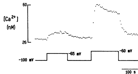
FIGURE 8 The influence of holding potential on intracellular [Ca^{2+}] . The fluorescence intensity at 380 nm excitation was recorded at 5-s intervals while the holding potential was changed. The fluorescence at 358 nm excitation was recorded \sim 30 s before and immediately after the sequence shown. The ratio F_{380}/F_{358} was formed for each point by interpolating between the two F_{358} values. The [Ca^{2+}] was calculated from the ratio with -R_{max} = -0.34 , -R_{min} = -1.91 , and K_D = 89 nM, the mean values from Table I. The upper panel shows the [Ca^{2+}] as the membrane potential was changed from -100 mV to -65 and -60 mV (depicted schematically in the lower panel). Fiber 410, 4.0 \mu\text{m} per sarcomere, 9^\circ\text{C} .
