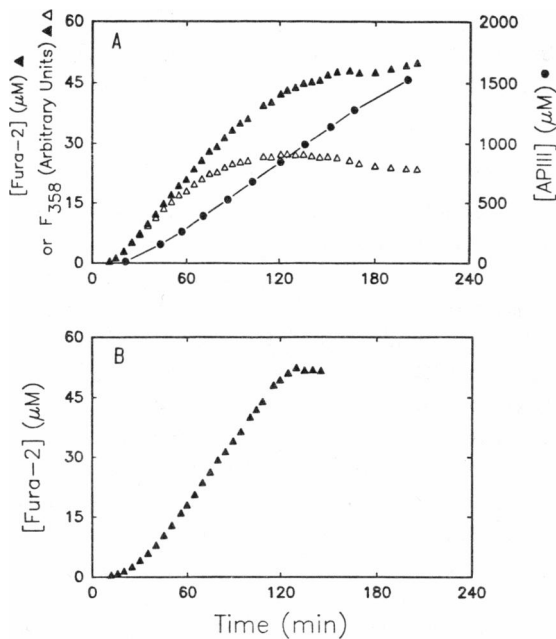
FIGURE 2 Time course of entry of AP III and fura-2 into muscle fibers. At time = 0, internal solution containing 50 \mu\text{M} fura-2 and 1 mM AP III (A) or 50 \mu\text{M} fura-2 and no AP III (B) was applied to the end-pools. Subsequently, the concentration of AP III and the emitted fluorescence at 358 nm excitation due to fura-2 ( F_{358} ) were measured in the central recording pool at various times. (A) Solid circles and right ordinate, concentration of AP III in the fiber in the central pool, calculated as described in the text. Open triangles, F_{358} measured from the fiber in the central pool (arbitrary scale). Solid triangles, F_{358} after correction for the absorption of incident and emitted light by AP III as described in the text. The solid triangles (and left ordinate scale) also give the concentration of fura-2 in the fiber calculated from the corrected F_{358} . Fiber VI217, 10°C, diameter 105 \mu\text{m} , 3.9 \mu\text{m} per sarcomere. (B) Concentration of fura-2 in another fiber exposed to fura-2 but no AP III in the end pools. In this case no correction was needed for AP III absorbance and the fura-2 concentration was calculated directly from the measured F_{358} by Eq. 6. Fiber VI237, 10°C, diameter 80 \mu\text{m} , 4.0 \mu\text{m} per sarcomere. The fiber membrane potential was held at 0 mV throughout the course of both experiments.
