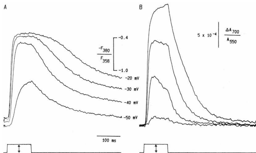
FIGURE 3 Comparison of simultaneously recorded fura-2 and AP III signals for depolarizing pulses of various amplitudes in a voltage-clamped skeletal muscle fiber. ( A ) Ratio signals ( R ) of fura-2 fluorescence at 380 nm excitation ( F_{380} ) to that at 358 nm excitation ( F_{358} ) for 100-ms pulses from -100 mV to the indicated membrane potential. Each signal is presented as -R . The changes in baseline levels of the signals indicate that the resting [\text{Ca}^{2+}] increased during the course of the recordings, from 13 to 27 nM using the calibration values in Fig. 6, legend. ( B ) Antipyrylazo III absorbance signals \Delta A_{700} at 700 nm recorded simultaneously with the fura-2 signals in A and corrected for changes in AP III concentration by dividing by the resting absorbance A_{550} due to AP III at 550 nm. The total absorbance signal at 700 nm was corrected for dye-independent intrinsic components by subtracting the simultaneously recorded 850 nm absorbance signal scaled by (850/700)^{1.2} (Melzer et al., 1986b). Each record in A and B is the average of four successive applications of the same pulse at 30- or 45-s intervals. The AP III concentration increased from 393 to 460 \mu\text{M} for the sequence in A and B while F_{358} increased by 8%. Fiber 377, 3.9 \mu\text{m} per sarcomere, 9.0°C.
