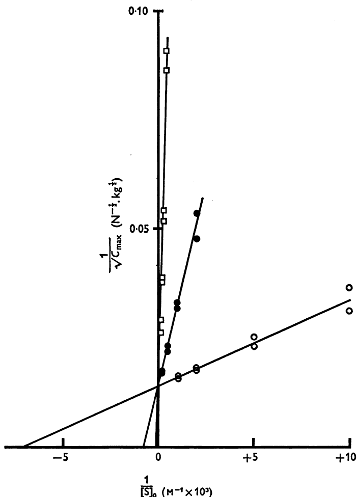
Fig. 5. 1/\sqrt{C_{\max}} for the contractures evoked by caffeine (○—○), naphazoline (●—●) and 1-methyl imidazole (□—□), in sodium-free fluid, are plotted against the reciprocal of the concentration of the substance in each case. The common intercept with the ordinate indicates a common mode of action for the three substances in the initiation of contraction. The intercept with the abscissa yields an estimate of the affinity constant for each compound. All the lines were obtained by regression analysis ( r > 0.98 and P < 0.01 ). 1 mM calcium; 17.0° C; Phosphate Ringer.
