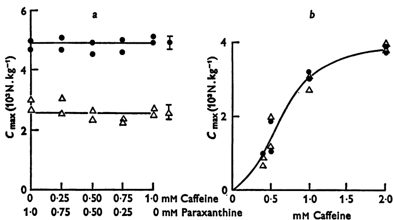
Fig. 3. The effects of mixing two active methylxanthines ( a ), and of mixing an active and an inactive methylxanthine ( b ), in sodium-free solutions, on the strength of the contracture induced by their application. a , compares the amplitude of the preceding sodium-free contracture (●—●) with the response induced by mixtures of caffeine and paraxanthine in which the total methylxanthine concentration was kept constant at 1 mM (△—△). Note that there is only a small variation in the amplitude of both types of response; the symbol on the left of each curve shows the mean \pm s.d. of all the results for each type of contracture. 1 mM calcium; 19.0° C; Tris Ringer. b , from another experiment. The dose-response curve for the caffeine contracture evoked after the spontaneous relaxation of a sodium-free contracture (●—●), is not altered by the presence of 1 mM 1,3,9-trimethylxanthine (△—△). Line drawn by eye. 2 mM calcium; 19° C; Tris Ringer.
