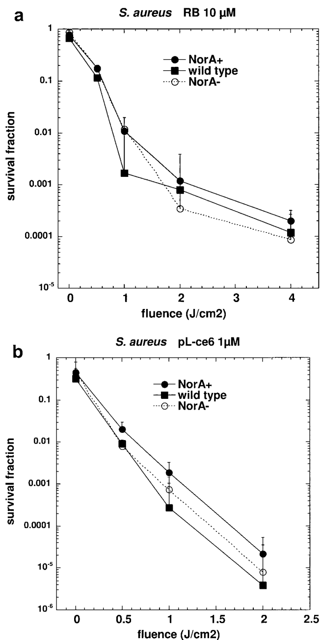
FIG. 6. Phototoxicity of (a) RB at 10 \mu\text{M} and (b) pL- c 6 at 1 \mu\text{M} , both with a wash with S. aureus NorA knockout (NorA - ), wild-type, and NorA-overexpressing (NorA + ) strains, followed by illumination with 100 mW cm -2 540-nm light for RB and 660-nm light for pL- c 6 .
