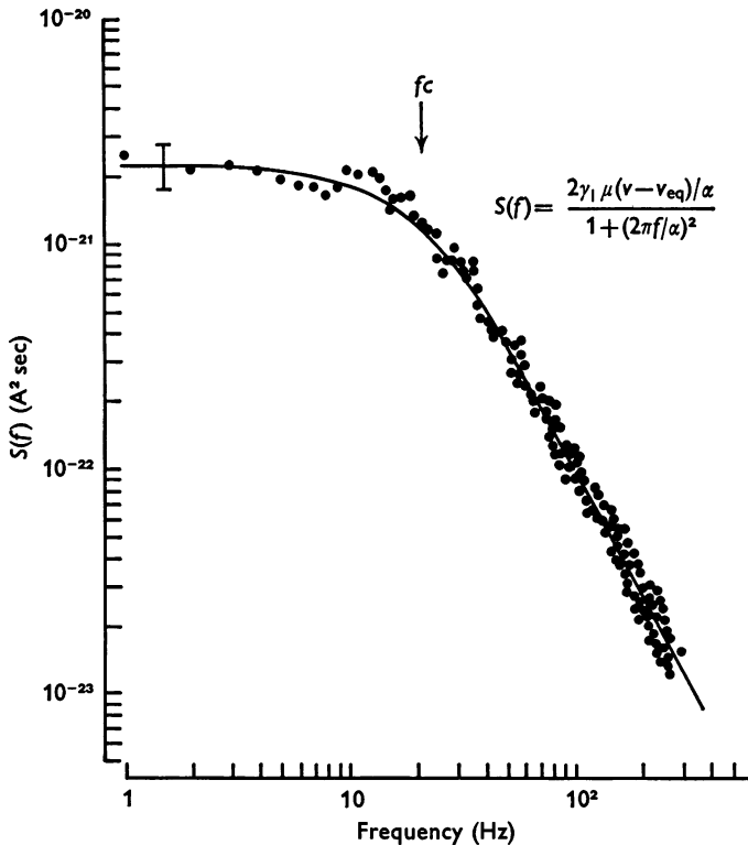
Fig. 4. Spectral density of e.p.c. fluctuations produced by a constant ACh iontophoretic application to a voltage-clamped ethylene glycol treated muscle end-plate. V = -60 mV, at 8^\circ\text{C} . The continuous line is the theoretical spectrum calculated from the model presented in the text (eqn. (4)) using the measured mean current ( \mu_1 = 80 \times 10^{-9} A), equilibrium potential ( V_{\text{eq}} = 0 ), \alpha = 0.132 msec ^{-1} , and assuming a single channel conductance \gamma = 0.32 \times 10^{-10} mhos. The cut-off frequency f_c = \alpha_s/2\pi = 21 HZ is indicated by an arrow. The error bar indicates \pm 1\sigma . The spectrum is based on 8192 digital samples taken at 1.02 kHz through a 300 Hz active low pass filter. This plot can be converted to a conductance fluctuation spectrum (units: mho ^2 -sec) by multiplying ordinate values by 1/(0.06)^2 .
