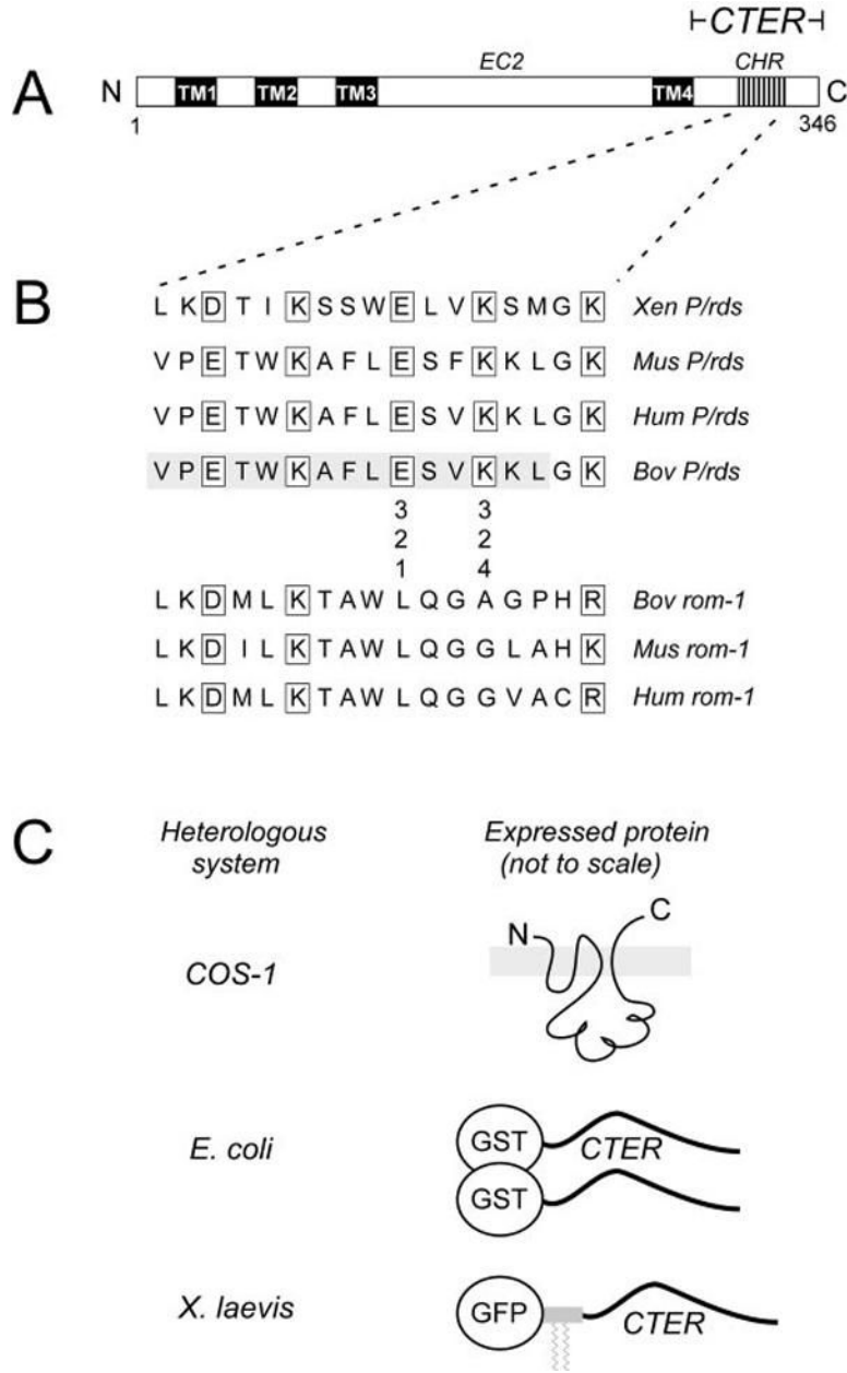
Fig.1. A, domain organization of P/rds. Four transmembrane domains (TM1-4) and the presence of several cysteine-containing motifs (not shown) in EC2 indicate a relationship within the tetraspanin family of proteins. CTER, C-terminal domain. B, alignment of the P/rds and rom-1 sequences for the predicted CHR at positions 312-328 within the 66-amino acid C-terminal domain. Conserved charged residues with three- to four-residue spacing are evident for P/rds. This study investigated the importance of the conserved charges at positions 321 and 324 for protein structure, localization, and fusogenic activity. Substitutions were guided by the aligned rom-1 sequences. The 15-amino acid bovine ( Bov ) P/rds region previously implicated as a fusion peptide is shaded. A recently reported localization signal (20) includes an additional five amino acids upstream and eight amino acids downstream of the X. laevis ( Xen ) sequence depicted. Mus , Mus musculus ; Hum , human. C, mutant P/rds variants expressed as 1) full-
