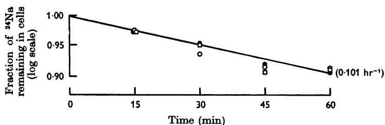
Fig. 15. The efflux of Na from low-Na, isotonicly resealed ghosts containing P_i but no ATP or ADP (cf. Figs. 13 and 14). The solution in which the ghosts were sealed contained (mM): P_i (pH 7.4) 4.6; Mg 5.5; Na 6.4; K 142; Cl 151; cysteine 1. The incubation media were the same as those used in the experiment of Fig. 14. At the end of the incubation the K-free medium contained 102 \mu\text{M-K} . \square , 10 mM-K medium; \circ , K-free medium; \bullet , K-free medium with ouabain. The figure in brackets is the rate constant for efflux.
