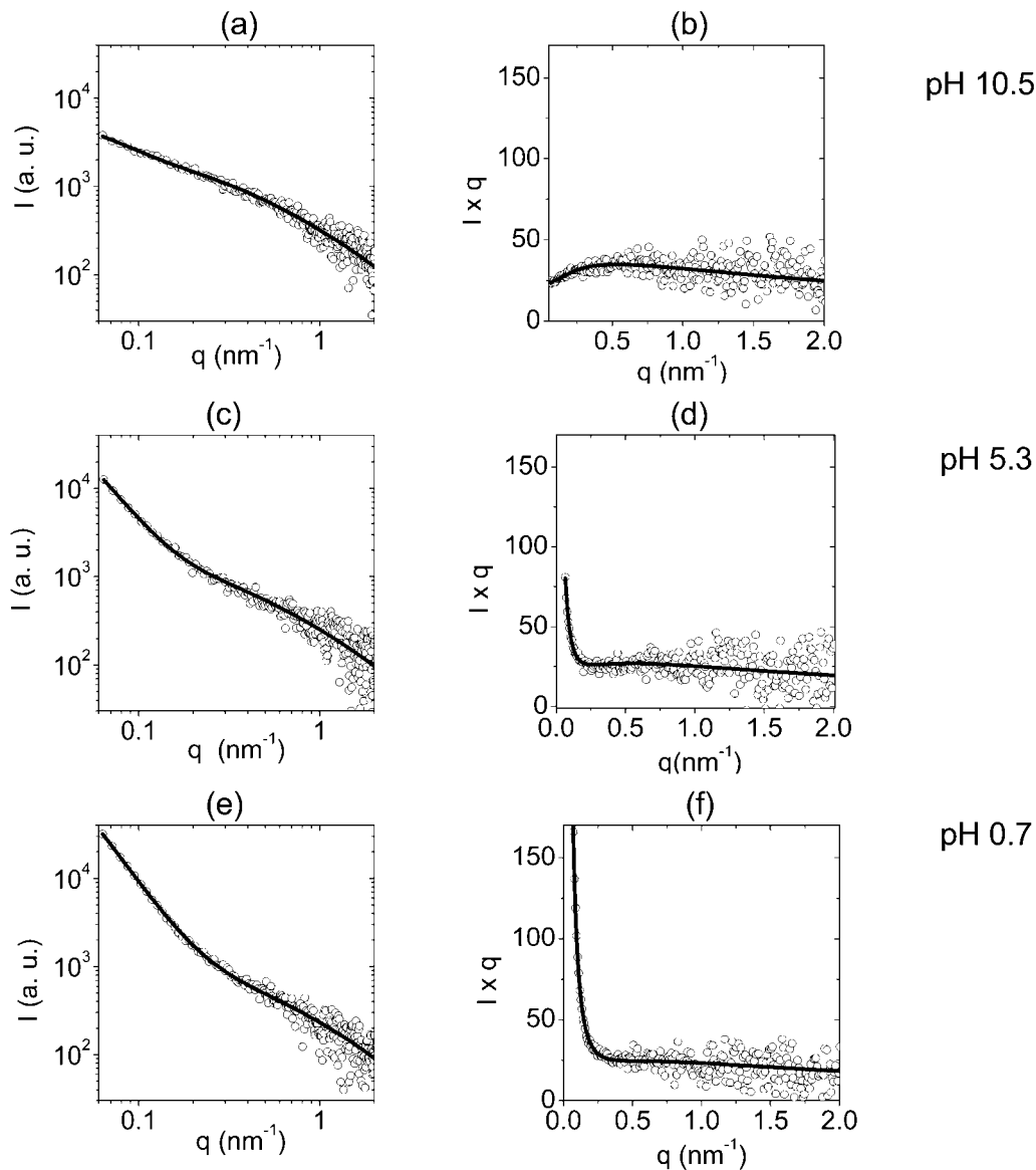
FIGURE 5 Log-log plots of scattering intensity of 0.4% EPS at different pH values are given in a , c , and e . Experimental data ( \circ ), and best fits to the experimental data with Eq. 4 ( \text{—} ), are given. The same data are shown on a Kratky-Porod ( I \times q versus q ) plot in b , d , and f . Both log-log and Kratky-Porod plots are given for three representative pH values. The parameters of the best fits are given in Table 2.
