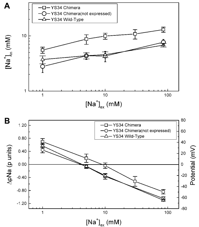
FIGURE 7 (A) [Na^+]_{in} versus [Na^+]_{ex} in cells expressing chimeric PomA/PotB7 E stators ( \square , eight cells) in cells containing the chimeric stator plasmid but grown without induced expression \circ , five cells) and in cells expressing wild-type MotA/MotB stators ( \triangle , five cells). (B) The same data as in A plotted as \Delta pNa versus [Na^+]_{ex} . Error bars indicate standard errors of the mean for each cell type and [Na^+]_{ex} .
