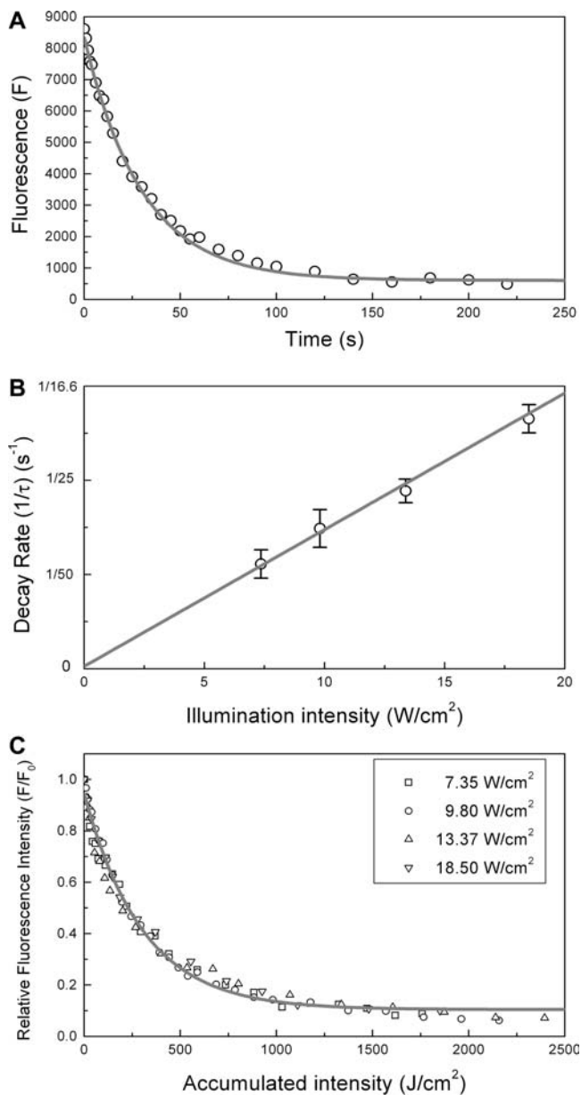
FIGURE 3 Photobleaching of Sodium Green. (A) Fluorescence intensity of a single loaded cell as a function of time during continuous illumination at an intensity of 9.8 W/cm 2 , exposure time 1 s. The curve is fitted as exponential decay with a time constant of 30 \pm 0.75 s. (B) Photobleaching decay rates as a function of illumination intensity (mean \pm SD of five cells at each intensity). The rates are proportional to intensity as expected for photobleaching (shaded line). (C) A combined decay curve for data at different intensities. Photobleaching can be described as F(x) = F_0 \exp(-x/x_0) , where x is the accumulated laser exposure.
