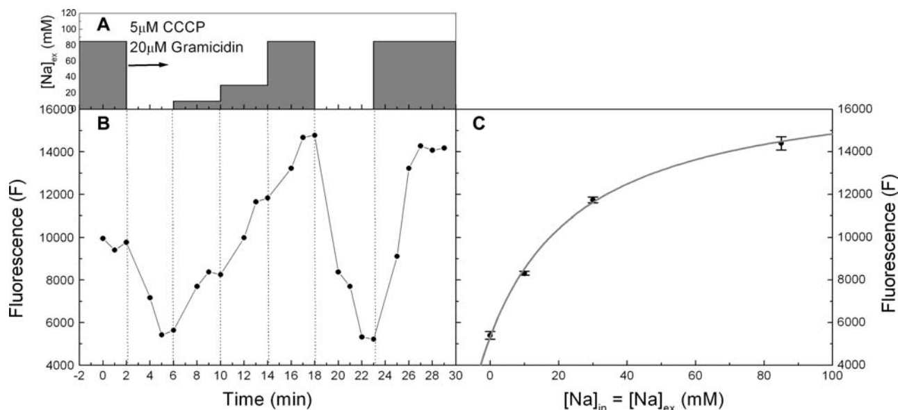
FIGURE 4 Calibration method. (A) [\text{Na}^+]_{\text{ex}} was varied between 0 and 85 mM with gramicidin and CCCP present to equilibrate the sodium concentrations across membrane. (B) Fluorescence intensity in response to changes of [\text{Na}^+]_{\text{ex}} ; \sim 3 min was required for equilibration of [\text{Na}^+]_{\text{in}} . (C) Steady-state fluorescence intensity as a function of sodium concentration, with a fit to Eq. 1. Mean \pm SD of three successive measurements of F are shown.
