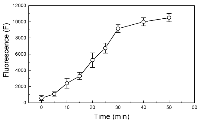
FIGURE 2 Fluorescence intensity of cells expressing chimeric motor proteins versus time of loading with 40 \mu M Sodium Green in motility buffer. The measurements were made immediately after loading; 30 min was chosen as the optimal loading time. Mean \pm SD of 10 cells is shown.
