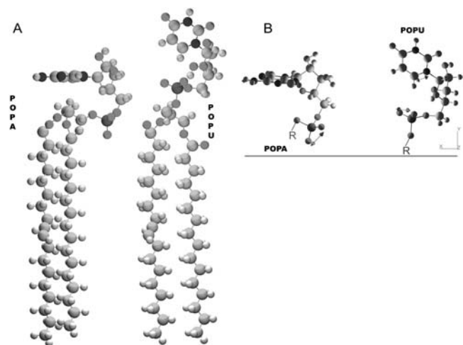
FIGURE 8 (A) POPA and POPU geometrical optimizations performed with Hyperchem 5.1 using AMBER force field. (B) This particular of the headgroup region highlights the transition moments considered above and their orientation with respect to the bilayer surface.
