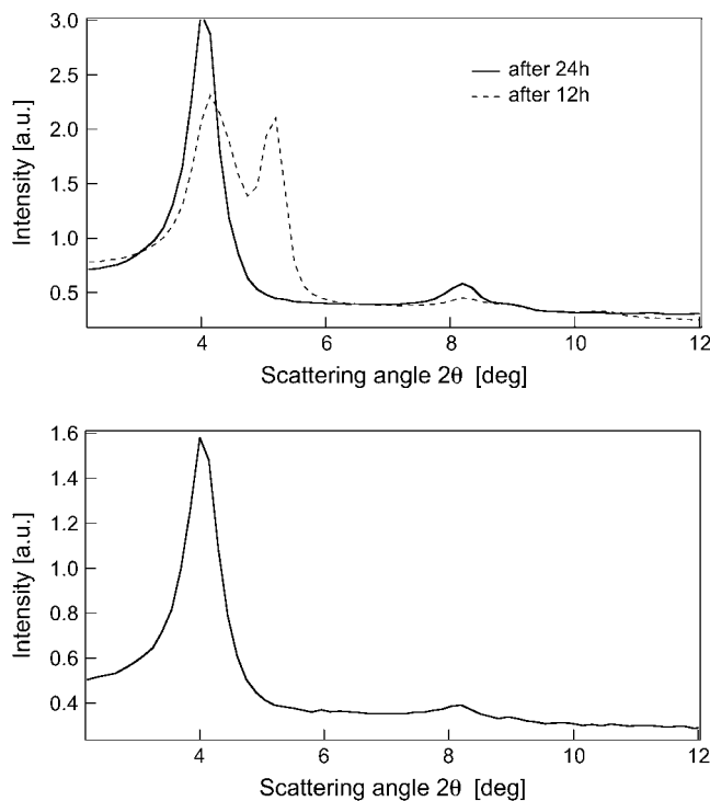
FIGURE 5 Diffraction patterns of POPA bilayers. (Top) 100% \text{D}_2\text{O} after 12 and 24 h of equilibration at 37^\circ\text{C} and 98% RH. (Bottom) 100% \text{H}_2\text{O} after 24 h of equilibration at 37^\circ\text{C} and 98% RH.
