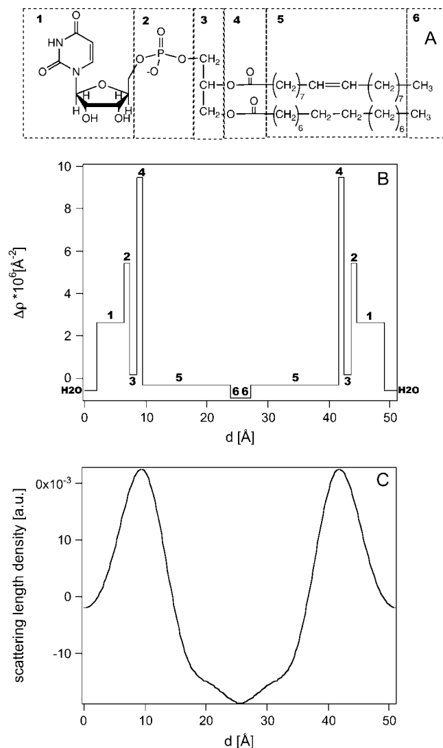
FIGURE 4 (A) Chemical structure of POPU in which we labeled each submolecular fragment that contributes to the scattering-length profile. (B) Calculated scattering-length profile evaluated by considering the contributions of different submolecular fragments as separated by sharp interfaces. (C) Experimental scattering-length density profiles at 0% \text{D}_2\text{O} in the direction normal to the membrane plane of the POPU sample.
