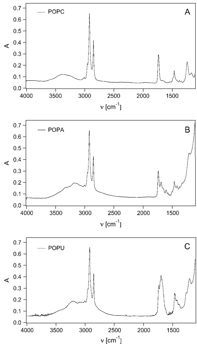
FIGURE 6 Infrared adsorption spectra of (A) POPC, (B) POPA, and (C) POPU bilayers.
