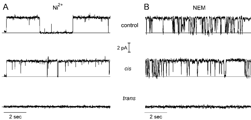
FIGURE 8 Effects of Ni 2+ and NEM on CLIC1. (A) Addition of 50 \mu M Ni 2+ to the cis and trans chambers of His-tagged channels reconstituted in 500 mM vs. 50 mM KCl in the presence of 1 mM DTT, HP +100 mV. Note the "alternative" gating mode shown in this example (see text). (B) Addition of 20 \mu M NEM to the cis and trans chambers of CLIC1 channels reconstituted in 500 vs. 50 mM KCl in the presence of 1 mM DTT, HP +100 mV. The DTT was removed by perfusion before making any additions. In each recording, the solid lines indicate the closed current levels.
