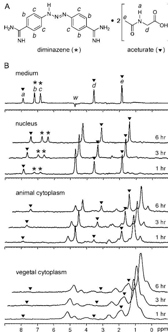
FIGURE 3 Drug uptake into cellular compartments. (A) Chemical structure of diminazene aceturate, with MR-visible protons labeled as a–e . Diminazene is labeled with an asterisk, and aceturate with inverted solid triangles. (B) Localized spectra of the external medium, the nucleus, the animal, and the vegetal cytosolic region of a prophase I-arrested stage VI oocyte in vivo, taken at different times after immersion in diminazene aceturate. Water peak referenced to 4.7 ppm. Intensity scale applies to all spectra. ( a , d , and e ) Aceturate ( \blacktriangledown ); ( b and c ) diminazene (*). The peak intensities of the diminazene peak c at 6.85 ppm and of the aceturate peak d at 3.55 ppm have been calculated for each compartment and after 1, 3, or 6 h, as the percentage of the respective peak intensity in the medium: nucleus, 15, 24, and 51 for peak c and 81, 84, and 95 for peak d ; animal, peak c not detectable, and 18, 36, and 38 for peak d ; vegetal, peak c not detectable, peak d at 1 h not detectable, and 3.2 and 6.2 at 3 h and 6 h, respectively.
