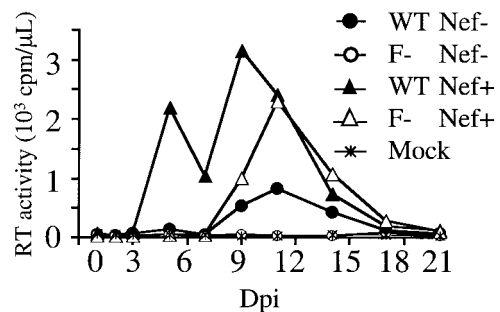
FIG. 9. Replication defect of F^- HIV-1 HXBc2 in PBMC is partially restored by wild-type nef . PBMC infected with 4 \times 10^4 RT cpm of Nef - HIV-1 HXBc2 (●), Nef - F^- HIV-1 HXBc2 (○), Nef + HIV-1 HXBc2 (▲), Nef + F^- HIV-1 HXBc2 (△), or supernatant from a mock transfection (×) were analyzed for RT activity at the indicated times. Dpi, days postinfection.
