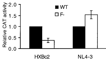
FIG. 8. Single-round infectivities of wild-type and F^- HIV-1 NL4-3 and HIV-1 HXBc2 . Levels of wild-type (WT) HIV-1 NL4-3 and wild-type HIV-1 HXBc2 required for 50% CAT activity, approximately 5 \times 10^6 RT cpm and 3 \times 10^7 RT cpm, respectively, were normalized to 1.0. The levels of F^- HIV-1 NL4-3 and F^- HIV-1 HXBc2 required for 50% activity are shown in comparison to their wild-type counterparts. Error bars represent the standard deviation of three independent infections.
