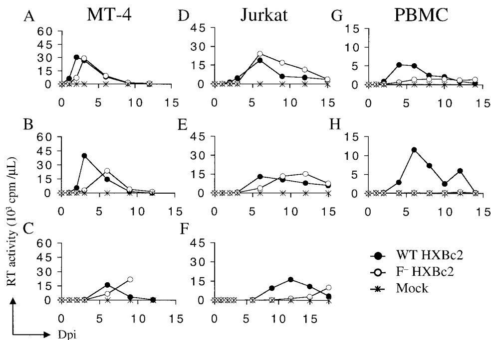
FIG. 3. F - HIV-1 HXBc2 displays a target cell type-dependent replication defect. Cells in panels A through H were infected with the same levels of wild-type (WT, ●) and F - (○) HIV-1 HXBc2 RT cpm as indicated for HIV-1 NL4-3 in Fig. 2, panels A to H. Other labeling is the same as in Fig. 2.
