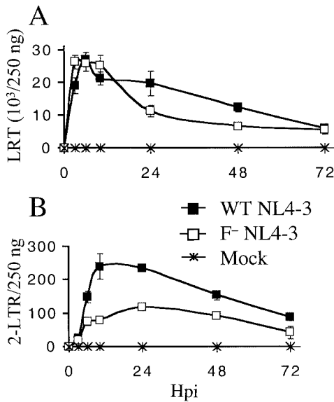
FIG. 5. cPPT-D mutation reduces the formation of HIV-1 NL4-3 2-LTR circles approximately twofold in Jurkat cells. (A) Cells infected with wild-type (WT) HIV-1 NL4-3 (■), F - HIV-1 NL4-3 (□), or supernatant from Env - transfections (×) were lysed at the indicated times, and 250 ng of total cellular DNA was assayed for total HIV-1 cDNA by RQ-PCR. (B) Cells infected with wild-type HIV-1 NL4-3 (■), F - HIV-1 NL4-3 (□), or mock-treated supernatant (×) were analyzed for levels of 2-LTR circles by RQ-PCR. Error bars represent variations between duplicate RQ-PCR assays. LRT, late reverse transcription; Hpi, hours postinfection.
