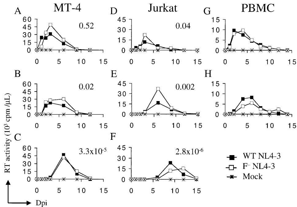
FIG. 2. F^- HIV-1 NL4-3 displays wild-type replication kinetics. (A) MT-4 cells infected with 10^6 RT cpm of wild-type (WT) HIV-1 NL4-3 (■), F^- HIV-1 NL4-3 (□), or supernatant from mock-transfected cells (×). (B) MT-4 cells infected with 4 \times 10^4 RT cpm of the viruses indicated in panel A. (C) MT-4 cells infected with 64 RT cpm of virus. (D through F) Jurkat cells infected with the levels of wild-type and F^- viruses indicated for MT-4 cells in panels A to C, respectively. (G and H) PBMC infected with 10^6 and 4 \times 10^4 RT cpm, respectively, of the indicated viruses. Numbers in panels A through F are multiplicities of infection for wild-type HIV-1 NL4-3 based on previously reported TCID 50 values (37). Dpi, days postinfection.
