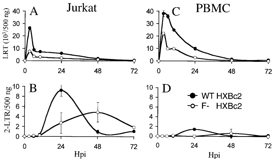
FIG. 6. F - HIV-1 HXBc2 supports wild-type level of 2-LTR circle formation in different cell types. (A) Jurkat cells infected with wild-type (WT) HIV-1 HXBc2 (●) or F - HIV-1 HXBc2 (○) virus were lysed at the indicated times, and 500 ng of total cellular DNA was assayed for total HIV-1 cDNA by RQ-PCR. (B) Cell lysates from panel A were analyzed for 2-LTR circle levels. (C) PBMC infected and processed as indicated for Jurkat cells in panel A. (D) 2-LTR circle levels of wild-type and F - HIV-1 HXBc2 in PBMC. Other labeling is the same as in Fig. 5.
