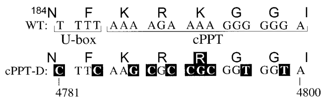
FIG. 1. Wild-type and mutant sequences. The central U-box and cPPT form part of the integrase coding region. Mutant sequences that differ from the wild-type (WT) sequence are highlighted by black boxes. Note that the cPPT-D mutation substitutes Arg for Lys-188 in the integrase. This change alone does not appear to impact integrase function, as HIV-1 LAI carrying just the K188R change replicated like the wild-type virus under conditions in which the HIV-1 LAI cPPT-D mutant was replication defective (50). Numbering is that for HIV-1 NL4-3 (1, 35).
