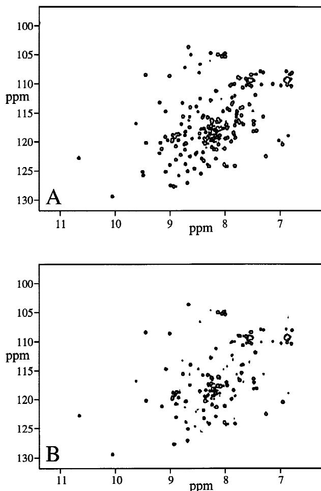
FIGURE 1. 2D (^{15}\text{N},^1\text{H}) -HSQC spectra of free and ribosome-bound E. coli IF3. The spectra of a 2-mM solution of ^{15}\text{N} -labeled IF3 were recorded in the absence (A) and in presence (B) of E. coli 30S ribosomal subunits at a stoichiometric ratio 30S/IF3 of 0.02%.
