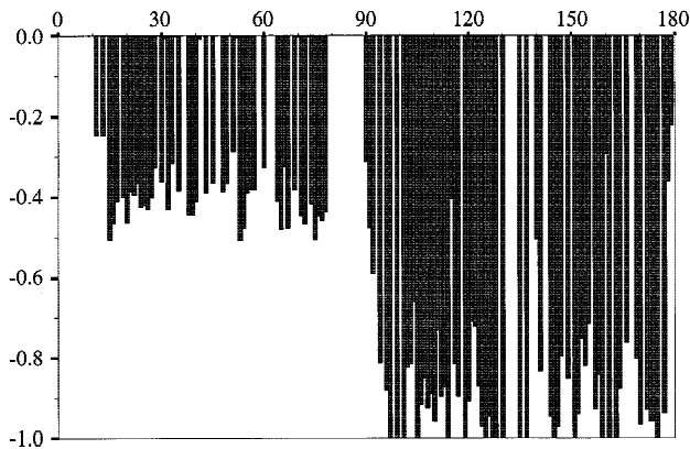
FIGURE 2. Effect of addition of 30S ribosomal subunits on the backbone amide resonances of the N-terminal and C-terminal domain of IF3. The figure shows differential intensity changes for the C-terminal and N-terminal domains. The position of each amino acid in the primary sequence of IF3 is indicated in the abscissa; the ordinate presents the relative intensity change, (V - V_0)/V_0 , of each assigned cross peak caused by the addition of E. coli 30S ribosomal subunits at a stoichiometric ratio 30S/IF3 of 0.02%. The blank slots correspond to residues for which the intensity could not be determined because of the absence of their signal (i.e., for Pro residues and in case of fast exchange) or because of severe overlap. Further experimental details are given in Materials and Methods.
