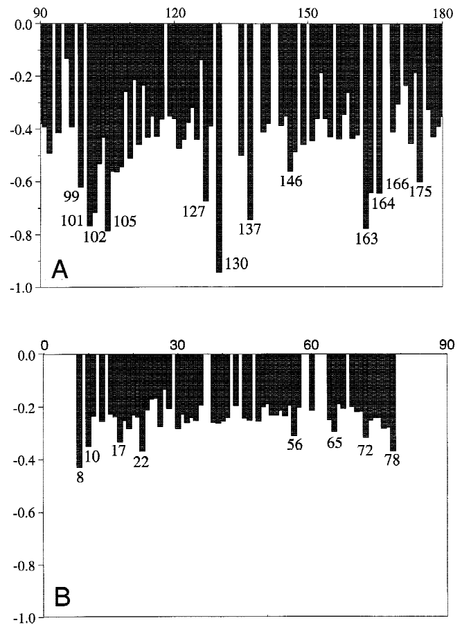
FIGURE 3. Intensity changes of individual backbone amide resonances of IF3 upon addition of 30S ribosomal subunits. A and B show the relative intensity change caused by successive additions of 30S ribosomal subunits for residues assigned to the C-domain (residues 90–180) and N-domain (residues 8–78) of IF3, respectively. The stoichiometric ratio 30S/IF3 was 0.002% for the data presented in A and 0.01% for B . The blank slots correspond to residues for which the intensity could not be determined because of the absence of their signal (i.e., for Pro residues and in case of fast exchange) or because of severe overlap. Further details are given in Materials and Methods.
