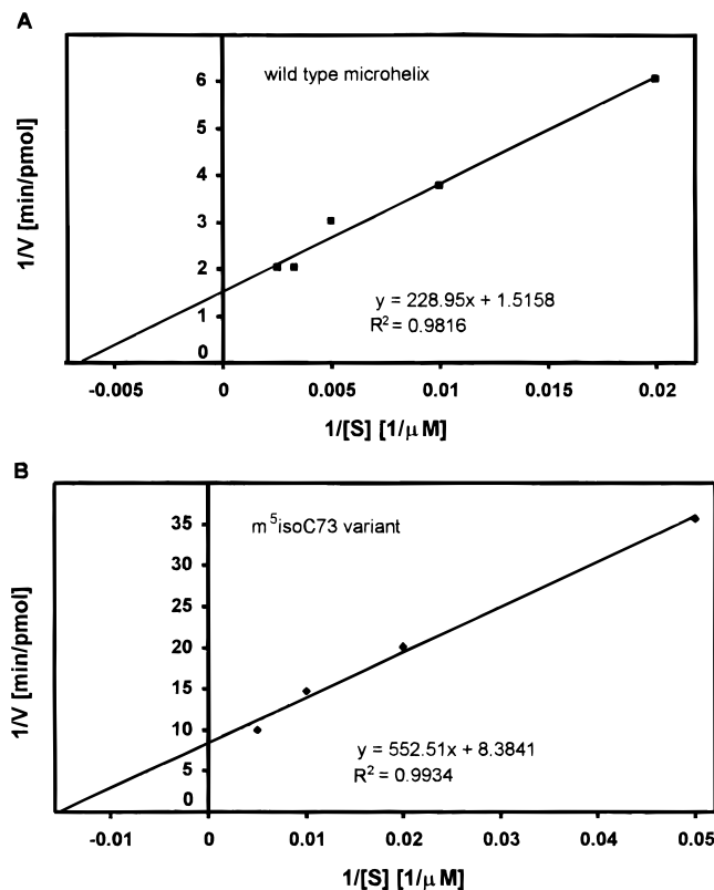
FIGURE 2. The Lineweaver–Burk plot of aminoacylation with cysteine of the wild-type RNA helix (A) and the m 5 isoC73 variant (B) as a function of substrate concentration. The linear regression of y = ax + b , together with the R^2 value (the correlation coefficient), is shown for each plot.
