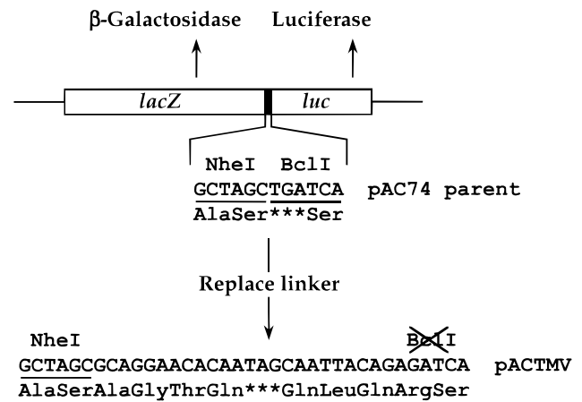
FIGURE 1. Schematic of the lacZ-luc reporter system. The reporter consists of tandem lacZ and luc genes separated by a short linker. The ends of the linker are NheI and BclI restriction sites that can be used to insert oligonucleotides bearing recoding sites. The figure shows the introduction of an oligonucleotide carrying the TMV termination readthrough site. When inserting such an oligonucleotide, the sequence of the BclI site was changed to eliminate an in-frame TGA termination codon that would otherwise block continued translation into luc .
