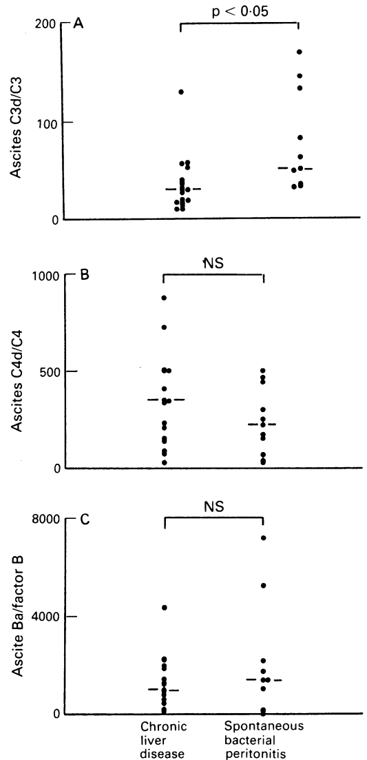
Figure 3: Complement activation as indicated by C3d/C3(A), C4d/C4(B), and Ba/factor B(C) in ascites of patients with spontaneous bacterial peritonitis and patients with severe chronic liver disease without infection.
