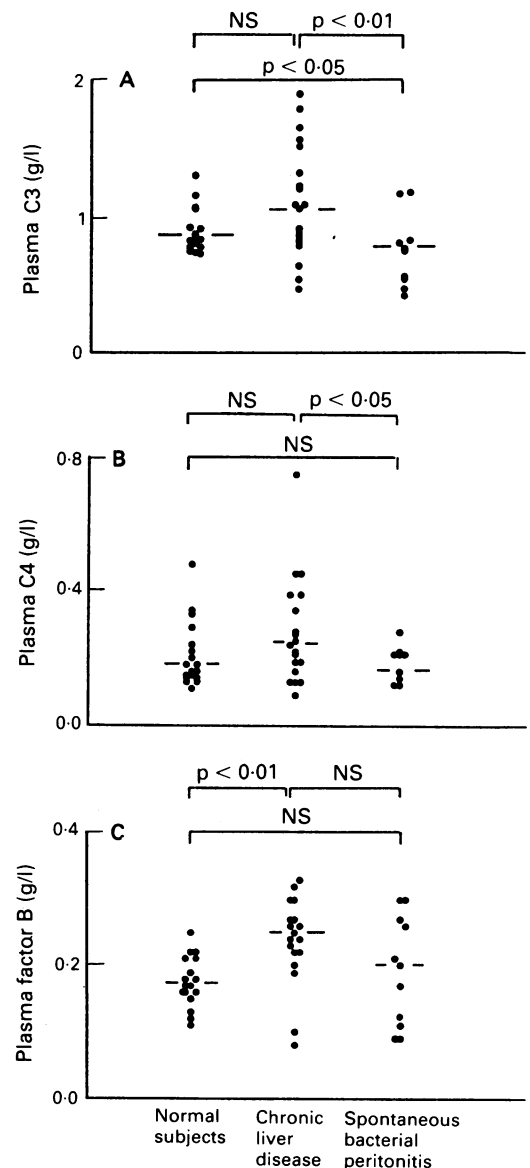
Figure 1: C3(A), C4(B), and factor B(C) in plasma of patients with spontaneous bacterial peritonitis, patients with severe chronic liver disease without infection, and normal subjects.
