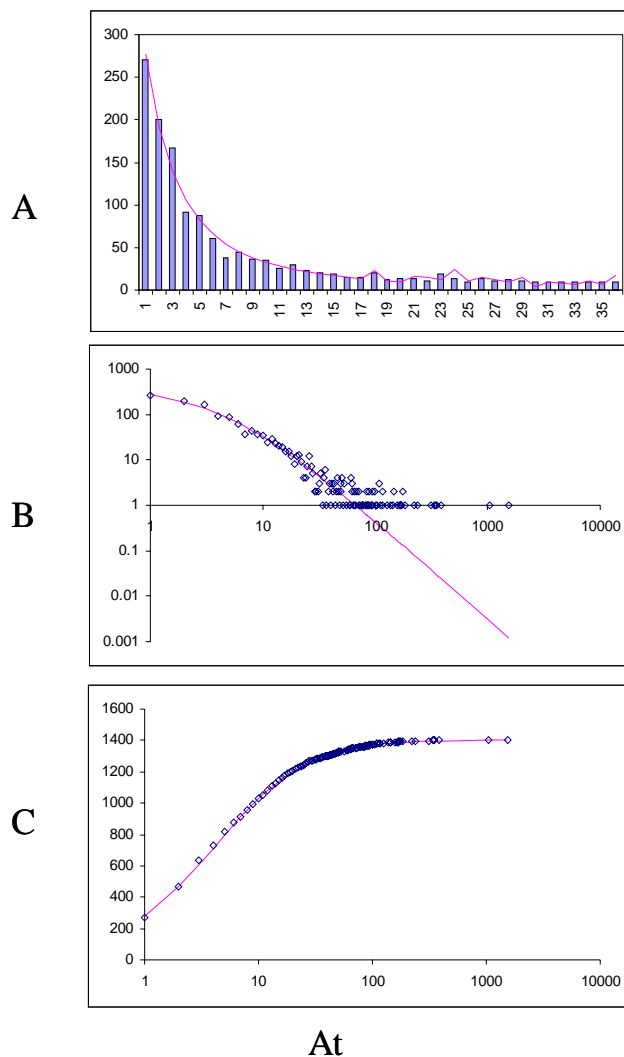
Figure 9 Fit of empirical domain family size distributions to the second-order balanced linear BDIM: the thale cress Arabidopsis thaliana . The panels and the designations are as in Fig. 6. B. Magenta line: f_i = 10750\Gamma(i+3.80)/\Gamma(i+5.98)
