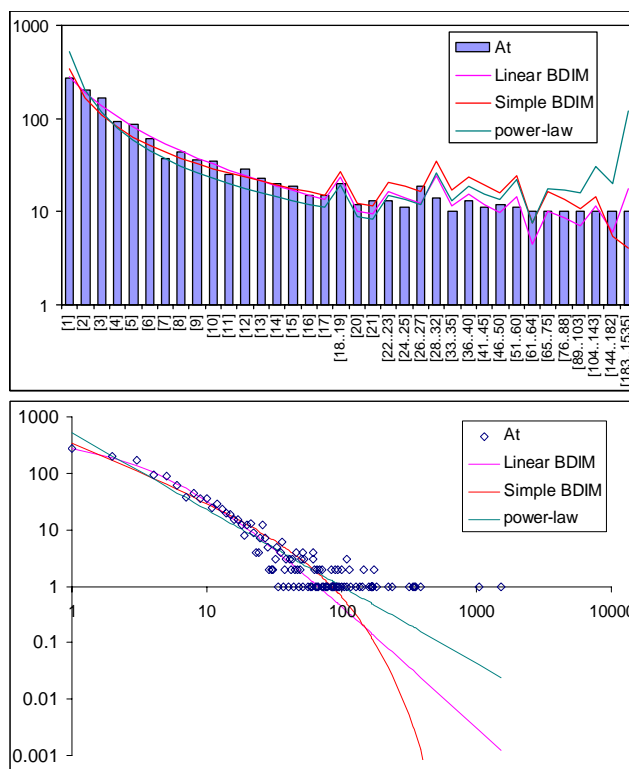
Figure 17 Comparison of different approximations of the empirical domain family size distribution: Arabidopsis thaliana . Magenta line: second-order balanced linear BDIM, f_i = 10750\Gamma(i+3.80)/\Gamma(i+5.98) , Red line: simple BDIM, f_i = 344 \times 0.98^i/i , Cyan line: power law, f_i = 516i^{-1.36} .
