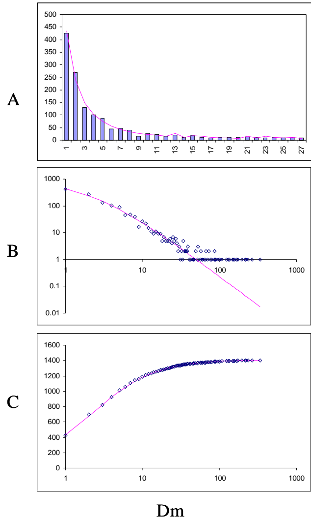
Figure 7 Fit of empirical domain family size distributions to the second-order balanced linear BDIM: the fruit fly Drosophila melanogaster . The panels and the designations are as in Fig. 6. B. Magenta line: f_i = 5258\Gamma(i+1.62)/\Gamma(i+3.79)
