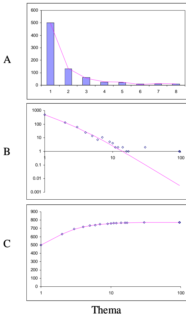
Figure 11 Fit of empirical domain family size distributions to the second-order balanced linear BDIM: the hyperthermophilic bacterium Thermotoga maritima . The panels and the designations are as in Fig. 6. B. Magenta line: f_i = 4256\Gamma(i+0.14)/\Gamma(i+3.22)
