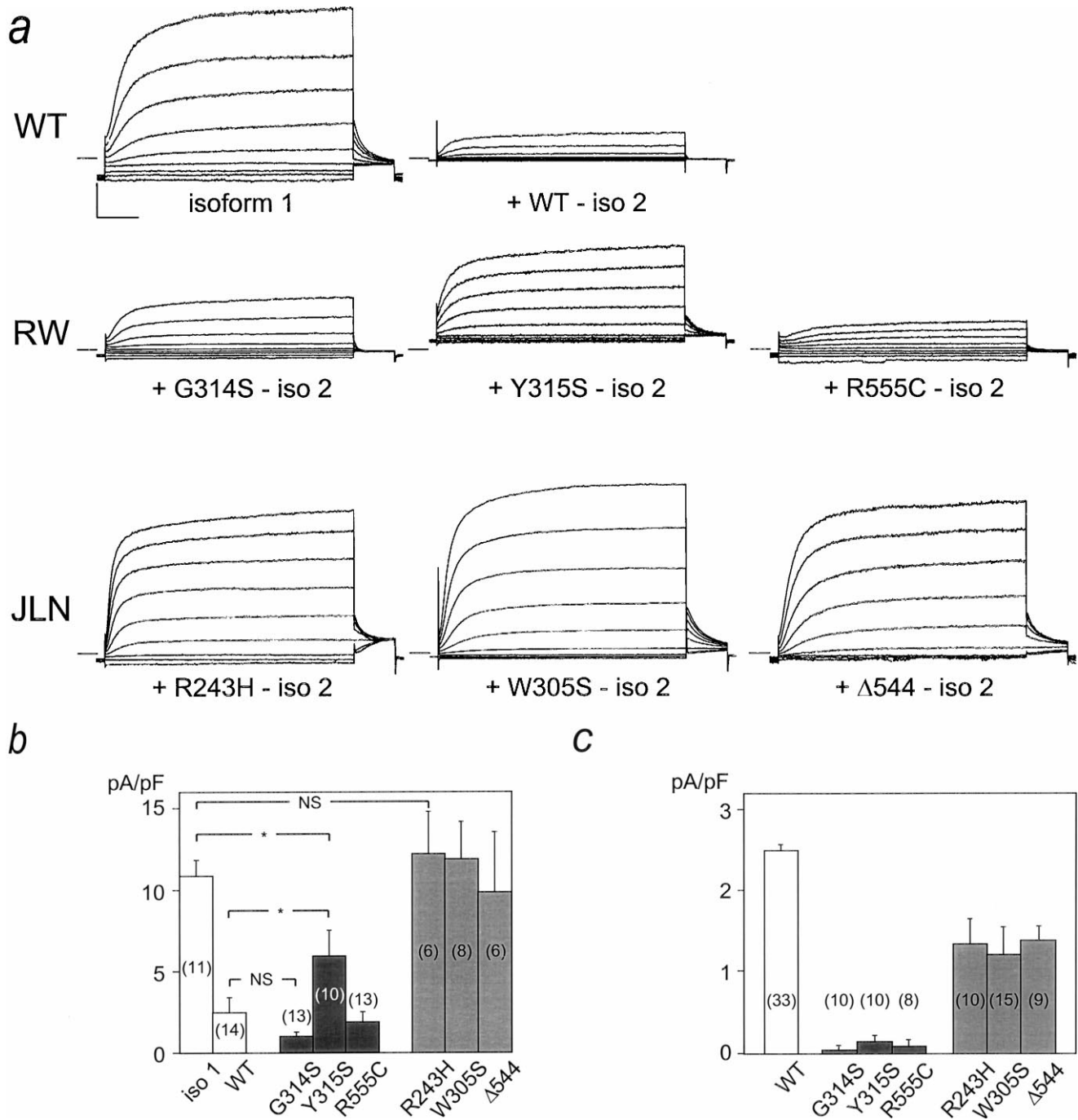
Figure 3 Expression of RW- and JLN-mutated KvLQT1 isoform 2 in the presence of IsK. a , K + currents recorded in COS-7 cells injected with wild-type (WT) isoform 1 (5 μg/ml) in the absence or presence of various isoform 2 constructs (2 μg/ml). Upper panel , Representative current tracings in cells injected with wild-type isoform 1 alone (isoform 1) and with wild-type isoform 1 plus wild-type isoform 2 (+ WT - iso 2) cDNA. Middle panel , Currents recorded with wild-type isoform 1 plus mutated RW (G314S, Y315S, R555C) isoform 2 cDNA. Lower panel , Currents recorded with wild-type isoform 1 plus mutated JLN (R243H, W305S, Δ544) isoform 2 cDNA. Voltage steps applied in sequence from -80 mV to various voltages in the range of -100 to +60 mV, and then to -40 mV where tail currents were recorded. Pulse duration was 3,000 ms. Current scale: 10 pA/pF; time scale: 500 ms. b , Averaged tail current amplitude in cells injected with isoform 1 (5 μg/ml) in the absence (iso 1) and presence of wild-type (WT) or mutated RW (G314S, Y315S, R555C) and JLN (R243H, W305S, Δ544) isoform 2 plasmids (2 μg/ml). Numbers between brackets indicate the number of cells tested. NS = nonsignificant; * P < .05 with standard t -test. c , Averaged tail current amplitude in cells coinjected with a plasmid combination made of wild-type isoform 1 (2.5 μg/ml), RW- or JLN-mutated isoform 1 (2.5 μg/ml), wild-type isoform 2 (1 μg/ml), and mutated RW or JLN isoform 2 (1 μg/ml). The open bar (WT) indicates current amplitude in cells injected with 5 μg/ml wild-type isoform 1 plus 2 μg/ml wild-type isoform 2. The dark gray bars indicate RW-mutated constructs, whereas the light gray bars indicate JLN-mutated constructs. Differences in the tail current amplitude between WT and RW- or JLN-mutated constructs or between RW and JLN constructs reached significance, with P < .01. In a , b , and c , all cells were coinjected with pCI-IsK (5 μg/ml). Injected plasmid concentration maintained constant at 15 μg/ml with pCI-GFP.
