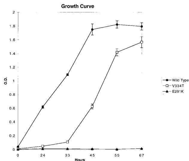
Figure 6 The V334T mutation in P. pastoris PEX13 attenuates its activity in vivo. Growth curves in minimal-methanol medium for P. pastoris pex13 \Delta strains carrying the PEX13 -expression plasmids pDC120 (wild-type; denoted by blackened circles), pDC120/E291K (inactive mutant; denoted by blackened triangles), and pDC120/V334T (denoted by unblackened squares). Data represent the average of three independent set of cultures, and the standard deviations are presented as brackets above and below data point.
