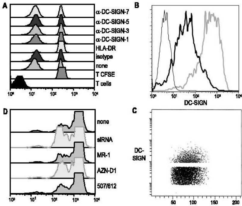
FIGURE 9. Inability of DC-SIGN to contribute to DC stimulation of the MLR. A , Immature DCs were pretreated for 20 min at room temperature with 20 \mu\text{g}/\text{ml} anti-DC-SIGN mAbs. DCs were cultured with allogeneic CFSE-labeled CD3 T cells at a ratio of 1:60. After 5 days, the presence of an MLR was documented by CFSE dilution. B , Immature DCs were transduced with siRNA DC-SIGN lentiviral vector or empty vector at an MOI of 20 and after 48 h were stained for DC-SIGN. The siRNA DC-SIGN (thick black line), empty vector (gray line), and isotype control (thin black line) are indicated. C , The low DC-SIGN-expressing cells were sorted and separated on a FACS. D , DC-SIGN low sorted immature DCs were used to stimulate an MLR as described in A , and additional anti-DC-SIGN mAbs were tested for inhibition of the MLR.
