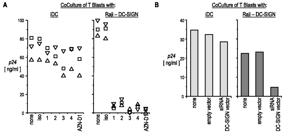
FIGURE 7. Effect of anti-DC-SIGN mAbs on HIV-1 transmission to T blasts. A , The indicated cells ( left panel , immature DCs; right panel , Raji-DC-SIGN) were incubated with anti-DC-SIGN mAbs as described in Fig. 6, and then infected with HIV-1 BaL in the continued presence of mAb. The cells were washed four times, and 5 \times 10^4 infected cells were cocultured with 10^5 T blasts. After 5 days, p24 secreted in the culture supernatants was quantified by ELISA. Each symbol corresponds to an individual experiment. B , DC-SIGN-expressing cells were transduced with siRNA lentiviral vector or empty vector at an MOI of 20, sorted for low DC-SIGN expression, and infected with HIV-1 before addition to T cells. The resulting cells were cocultured and assayed as described above.
