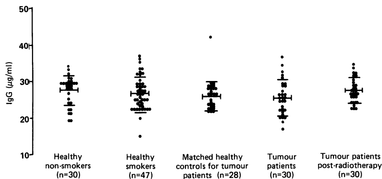
Figure 3: Bars show mean (standard error). No significant differences between groups, ( U=566 , p=0.144 , healthy smokers v controls).
