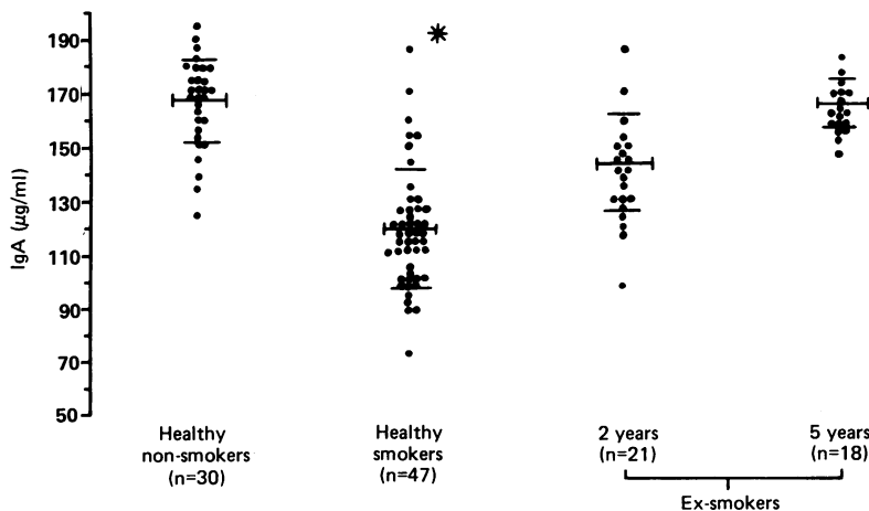
Figure 5: IgA concentrations in ex-smokers of 20 cigarettes daily, after 2 ( U=102.5 , p=0.0001 ), and 5 ( U=214 , p=0.633 ) years abstinence compared with controls. Current smokers are shown for comparison.
