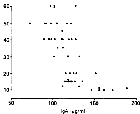
Figure 4: Relationship between daily cigarette consumption and salivary IgA concentration, r=-0.68 , p<0.00001 .
