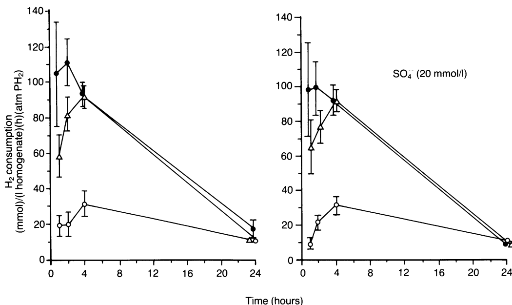
Figure 1: Hydrogen consumption (normalised for P_{H_2} ) by CH_4 producing faeces (●), non-methanogenic faeces (○), and by the mixture of the two types of faeces (△), during 24 hours of incubation with a gas space containing an initial H_2 concentration of 10%. The graph on the right shows the results obtained when the homogenates were supplemented with 20 mM Na_2SO_4 . Data are represented as mean (SEM).
