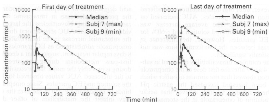
Figure 3 Median plasma concentration-time profiles measured on the first and last days of 8 days' oral treatment with 20 mg omeprazole as EC granules ( n = 10 ). The extreme profiles observed in individual subjects are also displayed.
