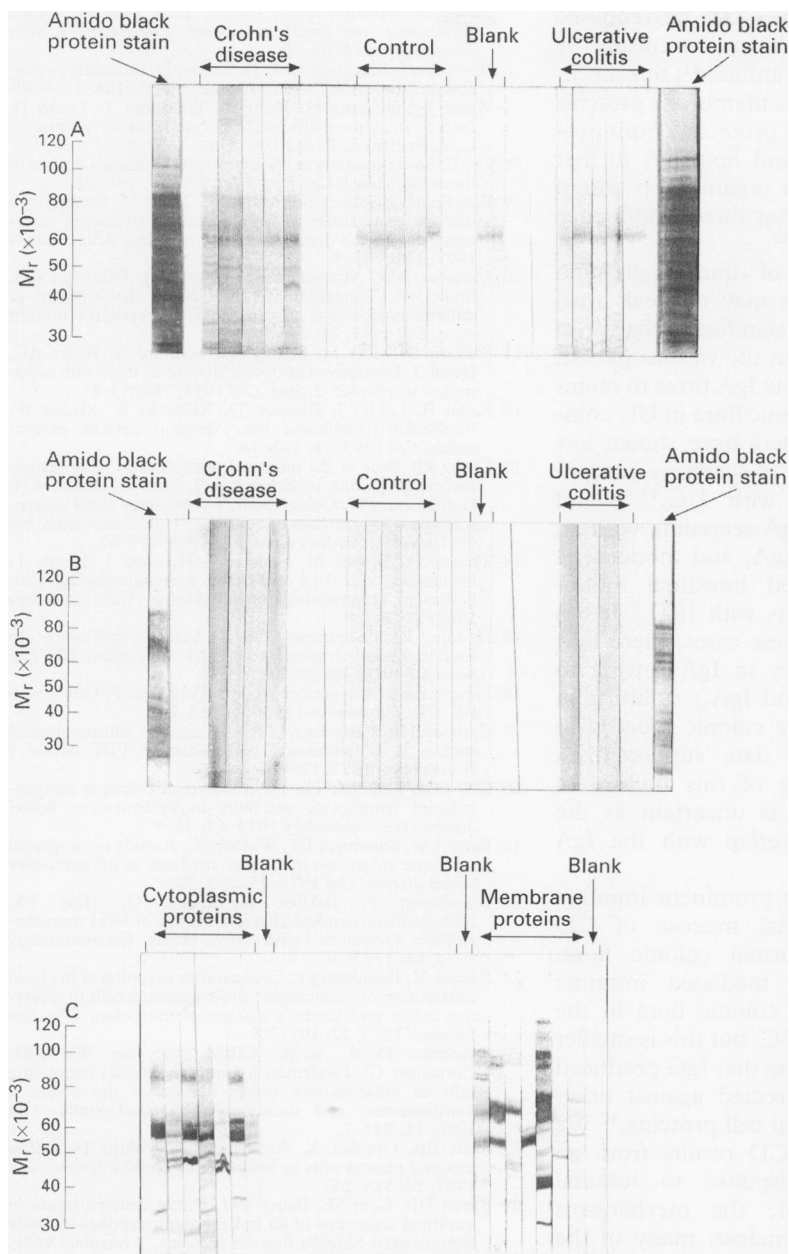
Figure 7: Binding of IgG from mucosal and serum immunoglobulins to E. coli cytoplasmic or membrane proteins. A western blot of E. coli cytoplasmic or membrane proteins was processed as shown in Figure 1, with each strip representing binding of a different patient mucosal or serum immunoglobulin sample. Binding is shown (A) by mucosal IgG (10 \mu\text{g/ml} ) to E. coli cytoplasmic proteins; (B) by mucosal IgG (10 \mu\text{g/ml} ) to E. coli membrane proteins; and (C) by control serum IgG (150 \mu\text{g/ml} ) to E. coli cytoplasmic and membrane proteins to strips cut from the same blots shown for (A) and (B). UC and CD serum samples gave similar results to those shown for (C). The biotinylated (antihuman IgG) secondary antibody also bound to a single E. coli cytoplasmic protein of M_r 59 000 (shown on the 'blank' strips where no mucosal immunoglobulin sample was added), showing that the band at M_r 59 000 in control and UC samples in (A) and (C) is due to crossreaction of this detecting antibody and not to mucosal or serum IgG binding.
