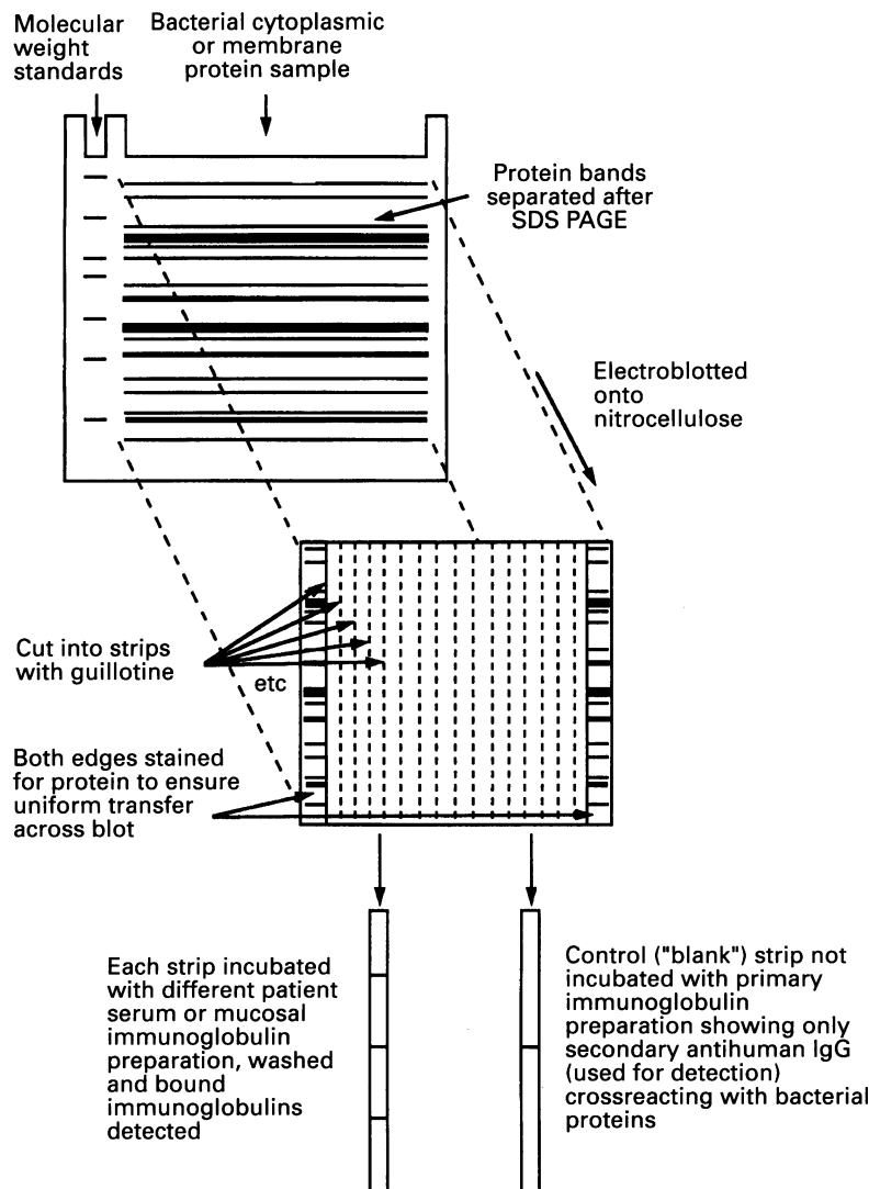
Figure 1: Method of assessment of mucosal and serum IgG binding to bacterial cytoplasmic or membrane proteins. Bacterial cytoplasmic or membrane proteins (200 µg) were run in a single large well by 12.5% SDS polyacrylamide gel electrophoresis. Molecular weight markers were run in a separate lane at the side of the gel and stained separately. The separated bacterial proteins were transferred to nitrocellulose, which was cut into strips, with each edge being stained for the bacterial protein bands with Amido black to ensure uniform transfer. Each intermediate strip was then incubated with either serum or mucosal immunoglobulin from an individual patient; after washing, specifically bound antibodies were detected using secondary biotin labelled antihuman IgG. Binding of secondary antibody independently of the mucosal or serum IgG was shown using 'blank' strips where no serum or mucosal immunoglobulin had been added.
