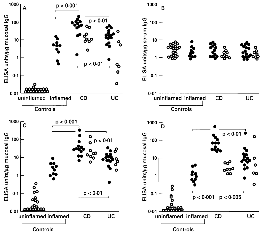
Figure 3: ELISA of binding by mucosal IgG from control and IBD patients against proteins of (A) and (B) E coli (C) Bacteroides fragilis , and (D) C perfringens . Plates were coated with a preparation containing cytoplasmic and membrane proteins of each non-pathogenic bacterial isolate. Serial dilutions of samples of mucosal immunoglobulins from each patient were tested, and bound immunoglobulins were detected with biotinylated polyclonal mouse antihuman IgG by avidin conjugated horseradish peroxidase activity. Calibration curves were run for each plate using dilutions of a standard serum calibrant of known high titre to each bacterial preparation. IgG ELISA units were calculated from the linear mid-portion of the curve (after subtraction of the blank without added mucosal or serum immunoglobulin) using the standard calibrant for that bacterial species. Results were expressed in IgG ELISA units per \mu\text{g} of total IgG. Inflamed controls (gastrointestinal infection, diverticulitis or ischaemic colitis) and active CD or UC are shown by filled circles. Irritable bowel syndrome controls or inactive IBD are shown by open circles.
