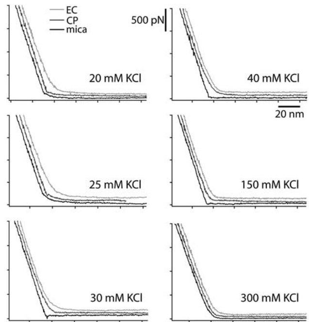
FIGURE 3 Force curves on the EC side ( light shaded ) and the CP side ( dark shaded ) of PM and on mica ( solid ) at different salt concentrations (20–300 mM KCl). The curves have been offset for better visibility. The maximum force applied by the tip is \sim 2 nN (500 pN force scale) corresponding to the force beyond which all the curves look similar when superimposed, regardless of the sample.
