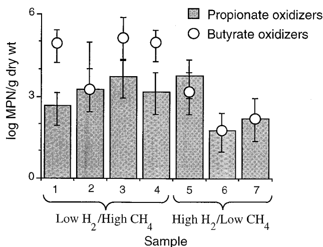
FIG. 6. Enumeration of fatty acid-oxidizing bacteria in high- and low-CH 4 -producing refuse samples. Error bars represent the 95% confidence limits. MPN, most probable number.
