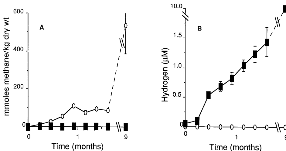
FIG. 3. Comparison of methane (A) and hydrogen (B) production in a methanogenic (O) and a nonmethanogenic (■) refuse sample. The error bars represent the standard deviations for duplicate incubations.
