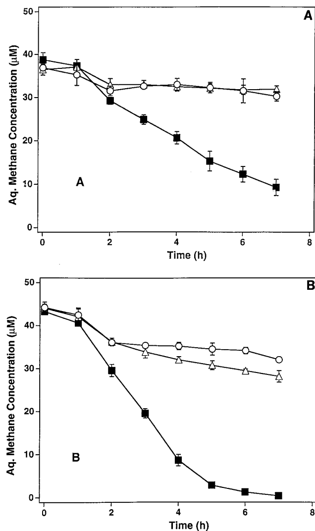
FIG. 2. Inhibition of methane oxidation by HCFC-21 in resting cell suspensions of M. capsulatus with sMMO (A) and pMMO (B). Symbols: ■, no HCFC addition; △, with 11 μM HCFC-21; ○, with 23 μM HCFC-21; □, autoclaved cell suspension without HCFC addition. Symbols represent the means of dissolved methane concentrations in three cell suspensions, and bars are \pm 1 standard deviation. Aq., aqueous.
