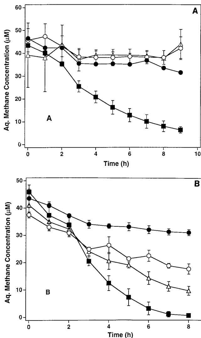
FIG. 1. Inhibition of methane oxidation by HCFC-22 in resting cell suspensions of M. capsulatus with sMMO (A) and pMMO (B). Symbols: ■, no HCFC addition; △, with 16 μM HCFC-22; ○, with 32 μM HCFC-22; ●, autoclaved cell suspension without HCFC addition. Symbols represent the means of dissolved methane concentrations in three cell suspensions, and bars are \pm 1 standard deviation. Aq., aqueous.
