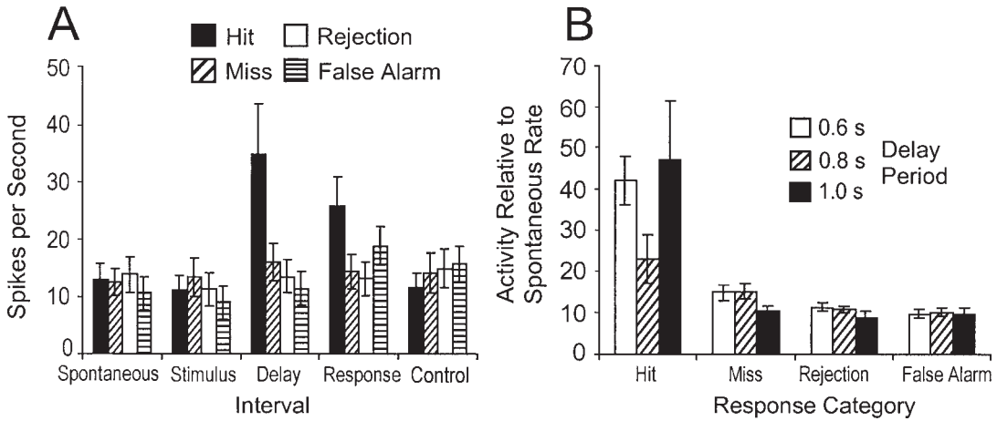
Fig. 5. Activity of 19 delay neurons during different time intervals of the DGNG task (A) and during the delay interval with different delay lengths (B). The neural activity of each unit was normalized to each unit's spontaneous activity (that equals one) and then to spikes per second, to compensate for the differences in the length of the intervals and the different number of trials for each neuron. A total of 310 hit, 179 miss, 452 correct rejection, and 34 false alarm trials were analyzed.
