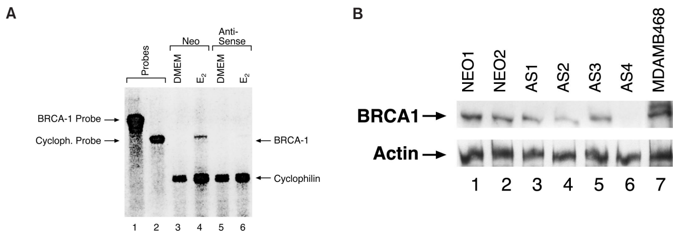
Expression of BRCA1 is reduced in BG-1 cells following infection with antisense BRCA1. (A) Ribonuclease protection analysis of BRCA1 mRNA. Lanes 1 and 2 show undigested probe for BRCA1 and loading control, cyclophilin. Lanes 3 and 4 are pooled BG-1 neo-infected control cells grown minus [Dulbecco's modified eagle medium (DMEM)] and plus (E 2 ) 10 -8 mol/l estrogen for 24 h. Lanes 5 and 6 are pooled BG-1 BRCA1 antisense-infected cells minus and plus 10 -8 mol/l estrogen, respectively, for 24 h. The observed doublet is the result of incomplete digestion. (B) Western blot analysis of individual control (NEO) and BRCA1 antisense (AS) clones. MDAMB468 is a BRCA1-positive breast cancer cell line.
