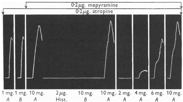
Fig. 2. Guinea-pig's ileum in 15 ml. Tyrode solution containing atropine 1 in 75,000,000. Effects of histamine (Hist.) and extracts from m. mucosae of dog's colon. A , untreated extract; B , extract after destruction of substance P by boiling in strong acid. The mg. refer to fresh weight of m. mucosae . After the second contraction, mepyramine 1 in 75,000,000. (For details see text.)
