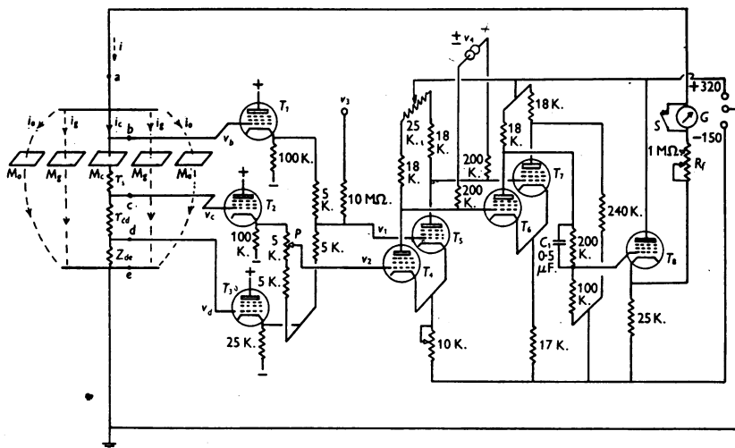
Fig. 6. Schematic diagram of feed-back amplifier. Screen resistances, grid stoppers and other minor circuit elements have been omitted. T_1 , T_2 , T_3 and T_4 are cathode followers; T_4 , T_5 , T_6 , T_7 and T_8 are d.c. amplifiers. All valves were 6AK5 except T_1 and T_2 which were 1223. G is a microammeter used in setting-up. S is a switch for short-circuiting G . M_c is the membrane in the central section of the guard system. M_g , membrane in guard channels. M_o , membrane outside guard system. i_c , i_g and i_o are currents through these elements. r_{cd} , fluid-resistance used to measure current ( 74 \Omega . at 20^\circ \text{C} ). r_s , resistance in series with membrane (about 52 \Omega . at 20^\circ \text{C} ). z_{de} , impedance of large earthed electrode and sea water between d and e . Potentials are given with respect to earth.
