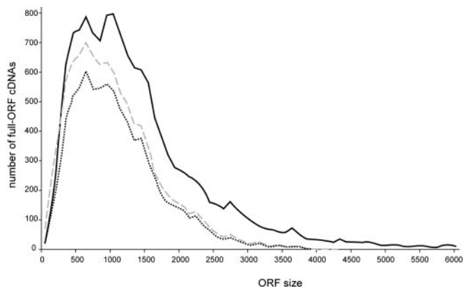
Fig. 3. ORF sizes of MGC full-ORF genes compared with RefSeq genes. The ORFs of MGC full-ORF genes and RefSeq genes were binned in 100-nt increments. The absolute numbers of MGC and RefSeq genes are compared for each size increment. RefSeq genes are represented by a solid line, the total of MGC genes is shown with the dashed lines, and MGC genes within the RefSeq set are depicted with dotted lines.
