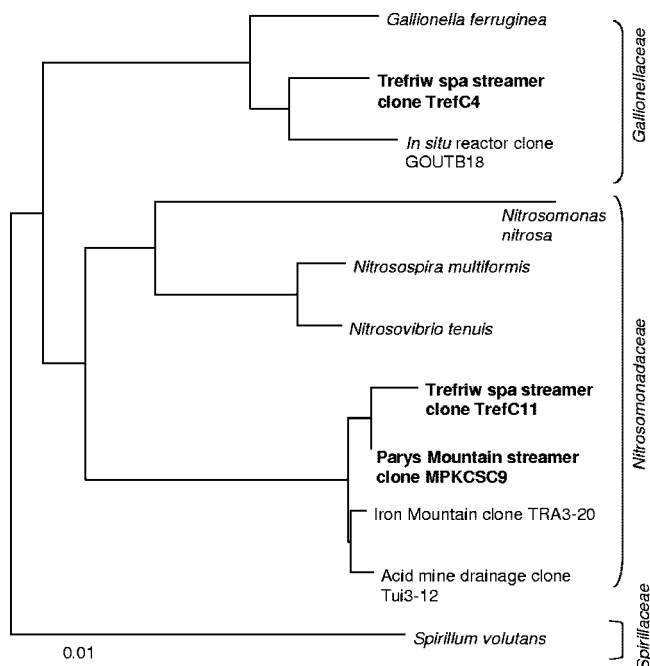
FIG. 3. Phylogenetic tree showing the relationship between the major clones identified in the Trefriw Wells Spa and Mynydd Parys acid streamers and other environmental clones and classified bacteria. Scale bar = 0.01 nucleotide substitution per site.
