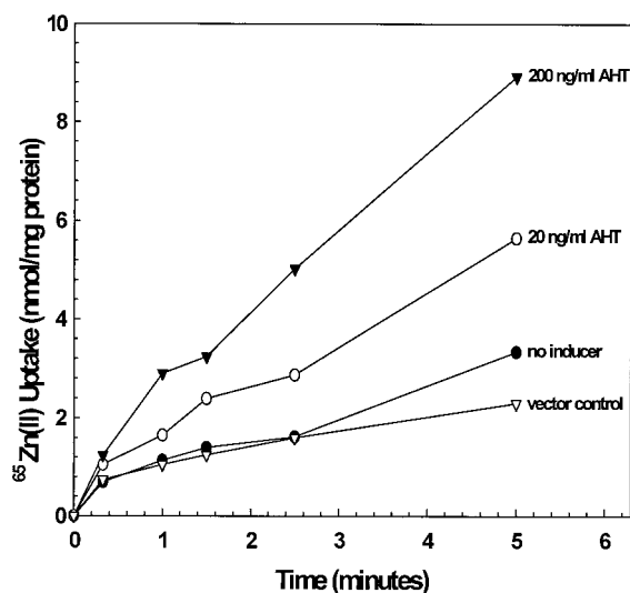
FIG. 3. Uptake of ^{65}\text{Zn(II)} by cells of E. coli GR362 ( \Delta znuABC \Delta zupT \Delta zntB::cam \Delta zitB zntA::kan ) expressing zupT . Cells were grown overnight in LB medium, diluted 50-fold into fresh prewarmed LB medium, and grown to an \text{OD}_{600} of 0.5, and expression of zupT was induced with 200 or 20 ng of AHT/ml for 10 min or not induced. The cells were washed with buffer A (10 mM Tris-HCl [pH 7.0], 2 g of glucose/liter, 10 mM \text{Na}_2\text{HPO}_4 ) and resuspended in the same buffer. ^{65}\text{ZnSO}_4 was added to a final concentration of 10 \mu\text{M} . The cells were incubated at 37°C, and 0.1-ml aliquots were filtered through nitrocellulose membranes (pore size, 0.45 \mu\text{m} ) at various times and immediately washed with 10 ml of buffer B (10 mM Tris-HCl [pH 7.0], 10 mM \text{MgCl}_2 ). The membranes were dried, and radioactivity was measured using a liquid scintillation counter. The protein concentration was determined using the method of Lowry et al. (11), and the amount of Zn(II) per milligram of protein was calculated. ●, E. coli GR362 ( \Delta znuABC \Delta zupT \Delta zntB::cam \Delta zitB zntA::kan )(pZUPT) (no inducer); ○, E. coli GR362 ( \Delta znuABC \Delta zupT \Delta zntB::cam \Delta zitB zntA::kan )(pZUPT) (20-ng/ml AHT); ▼, E. coli GR362 ( \Delta znuABC \Delta zupT \Delta zntB::cam \Delta zitB zntA::kan )(pZUPT) (200 ng/ml); ▽, E. coli GR362 ( \Delta znuABC \Delta zupT \Delta zntB::cam \Delta zitB zntA::kan )(pASK-IBA3).
