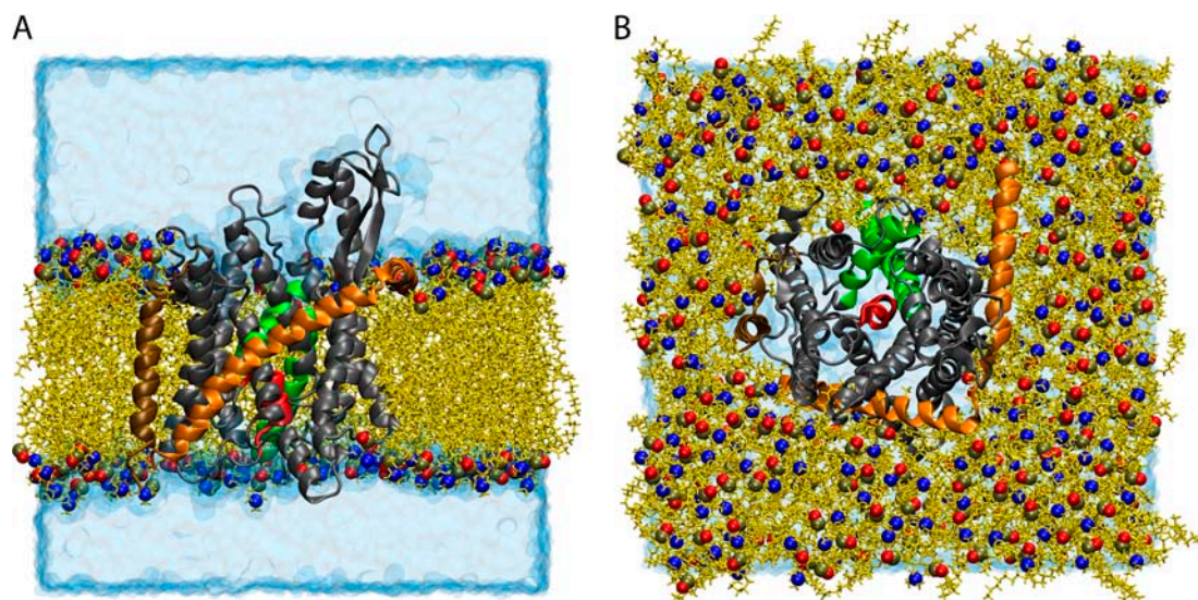
FIGURE 1 Simulated system of SecYE \beta in a lipid bilayer/water environment. SecYE \beta is shown in cartoon representation with SecY, SecE, and Sec \beta colored in gray, orange, and ochre, respectively. The plug, transmembrane domain 2a of SecY (residues Ile 55 to Gly 65 ) is presented in red, and TM2b (residues Gly 76 to Ser 91 ) and TM7 (residues Asn 256 to Gly 280 ) are shown in green (both also of SecY). The lipids are seen in yellow licorice representation with the phosphorus, nitrogen, and an oxygen of the headgroup highlighted as spheres colored in tan, blue, and red, respectively. The water box is drawn in transparent blue surface representation. (A) Side view of the simulated system. To display the protein more clearly, some lipids and water molecules have been removed, leaving a flat outward face. (B) Top view of the simulated system. The top solvation layer has been removed.
