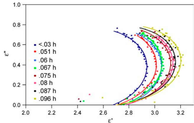
FIGURE 5 Cole-Cole plot for low hydrations. Lines are drawn to guide the eye.
