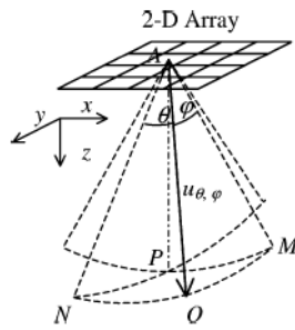
Fig. 17. The coordinate system of an ultrasound beam u_{\theta, \phi} generated by 2-D linear array with beam steering angle \theta in the xz -plane, which is equal to angle NAO and PAM , and beam steering angle \phi in the yz -plane, which is equal to MAO and PAN .
