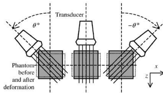
Fig. 4. Simulation model for strain tensor estimation. A linear transducer rotates for every 1^\circ around the center of the phantom, from -45^\circ to 45^\circ . RF signals are generated for each location of the transducer before and after phantom deformation.
