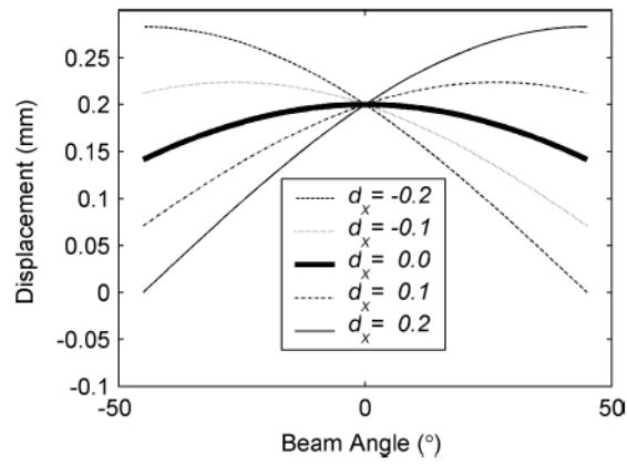
Fig. 3. Plots of projections of the actual displacement vector onto a unit vector in the \theta direction for an axial displacement of d_z = 0.2 mm and different values of the lateral displacement d_x in millimeters.
