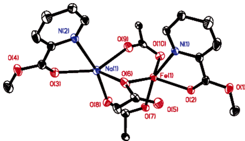
Figure 1. ORTEP diagram of [\text{NaFe}(\text{PIC}_2\text{DET})(\mu\text{-O}_2\text{CTrp})_3] ( 2 ) showing 30% probability thermal ellipsoids for all non-hydrogen atoms. Ligand 1 and the triptycene units of the bridging carboxylates are abbreviated for clarity. Selected interatomic distances (Å): Fe1 \cdots Na1, 3.181(2); Fe1-N1, 2.196(3); Fe1-O2, 2.184(3); Fe1 \cdots O5, 2.604(4); Fe1-O6, 2.131(3); Fe1-O7, 2.039(3); Fe1 \cdots O9, 2.320(4); Fe1-O10, 2.181(4); Na1-N2, 2.508(4); Na1-O3, 2.348(4); Na1-O6, 2.308(4); Na1-O8, 2.282(4); Na1-O9, 2.285(4).
