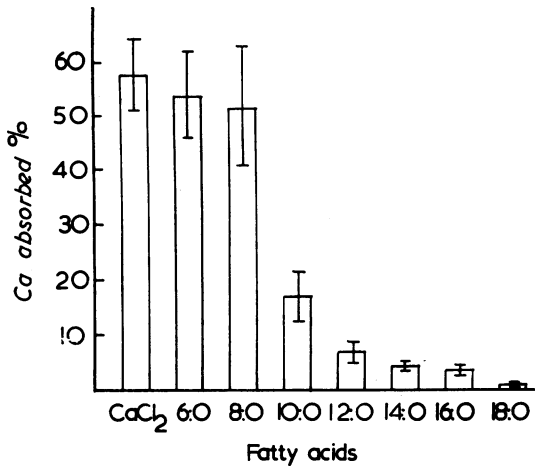
Fig. 1 Calcium absorption from the Ca-soaps of saturated fatty acids. Mean \pm SD.
