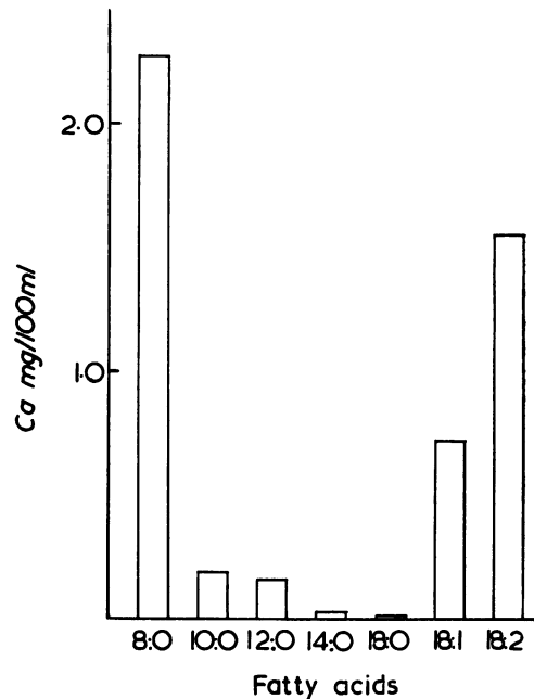
Fig. 3 Solubility of Ca-soaps in 0.02M Na-tauroglycocholate.
