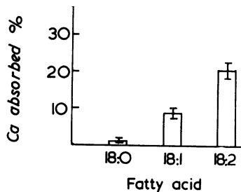
Fig. 2 Effect of unsaturation of fatty acids on the calcium absorption from their Ca-soaps. Mean \pm SD.
