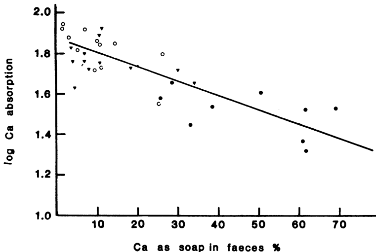
Fig. 4 Relationship between calcium absorption and the percentage of calcium as soap in the faeces after intragastric administration of \text{CaCl}_2 with stearic acid (●), glycerol tristearate (○), and glycerol trioleate (▼). ( r = 0.82 , P < 0.001 ).
